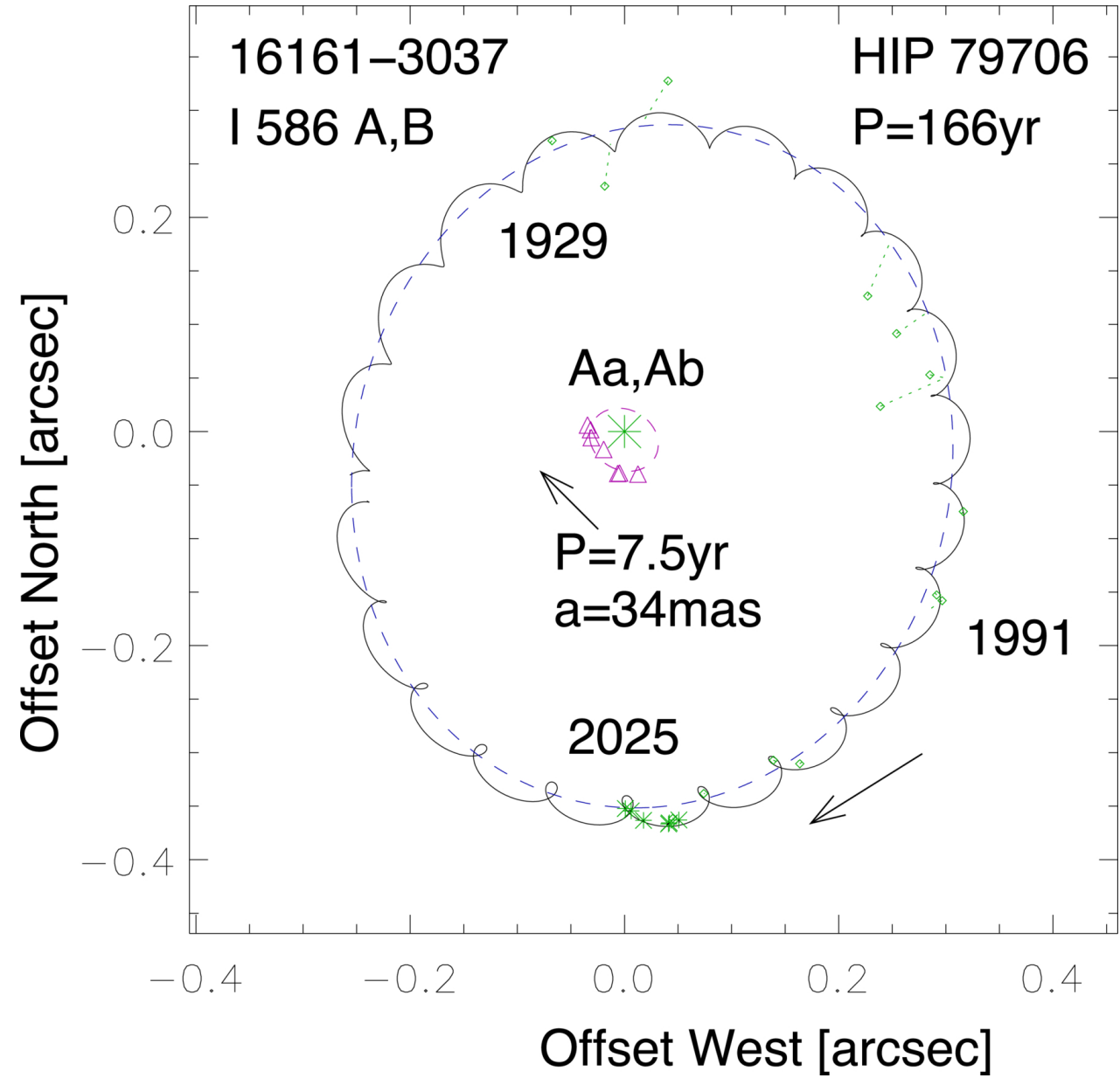
Figure 9. from Andrei Tokovinin 2026 Astron. J. 171 doi:10.3847/1538-3881/ae2fe6 https://dx.doi.org/10.3847/1538-3881/ae2fe6 © 2026. The Author(s). Published by the American Astronomical Society.
