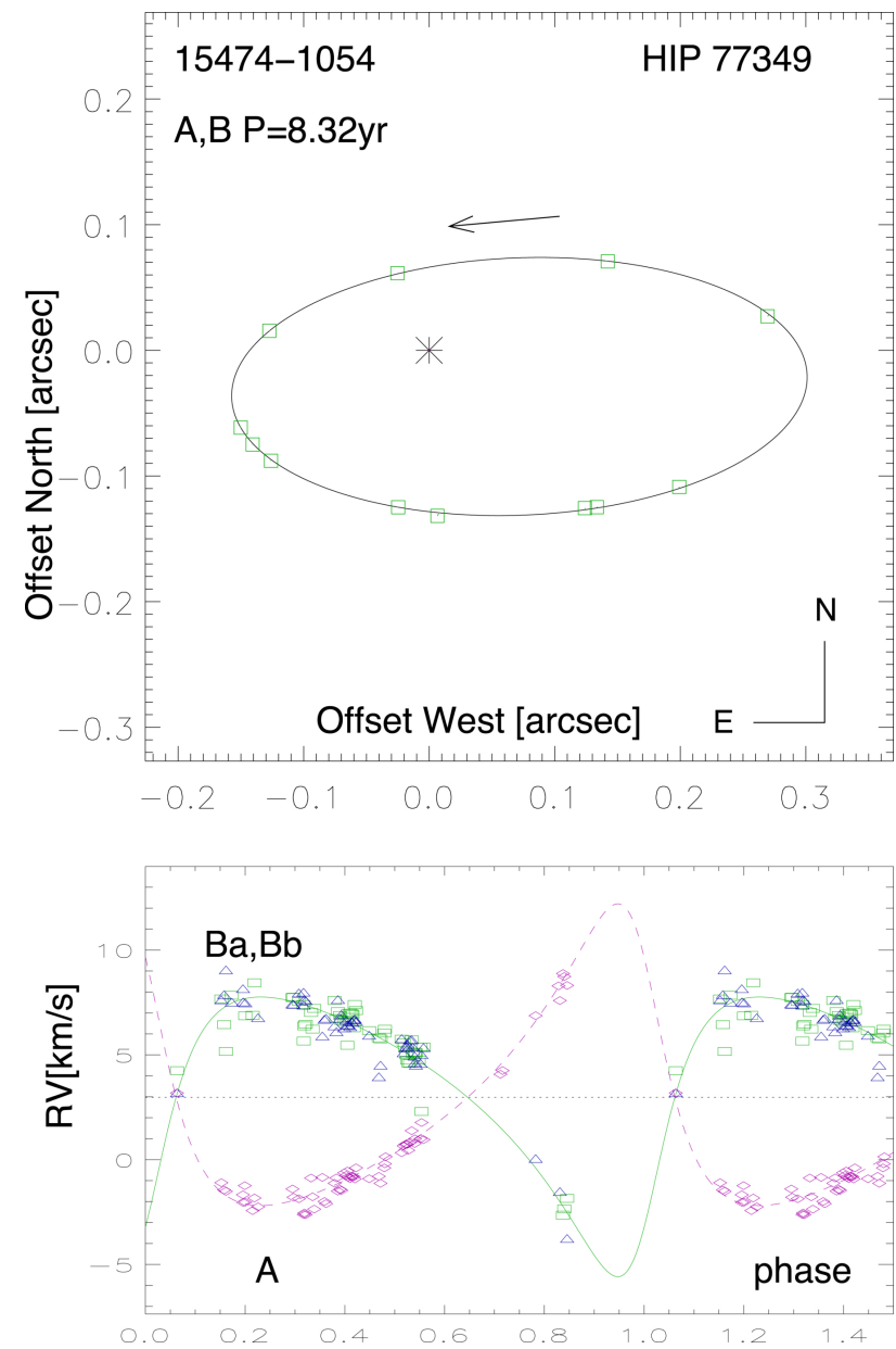
Figure 8. from Andrei Tokovinin 2026 Astron. J. 171 doi:10.3847/1538-3881/ae2fe6 https://dx.doi.org/10.3847/1538-3881/ae2fe6 © 2026. The Author(s). Published by the American Astronomical Society.
