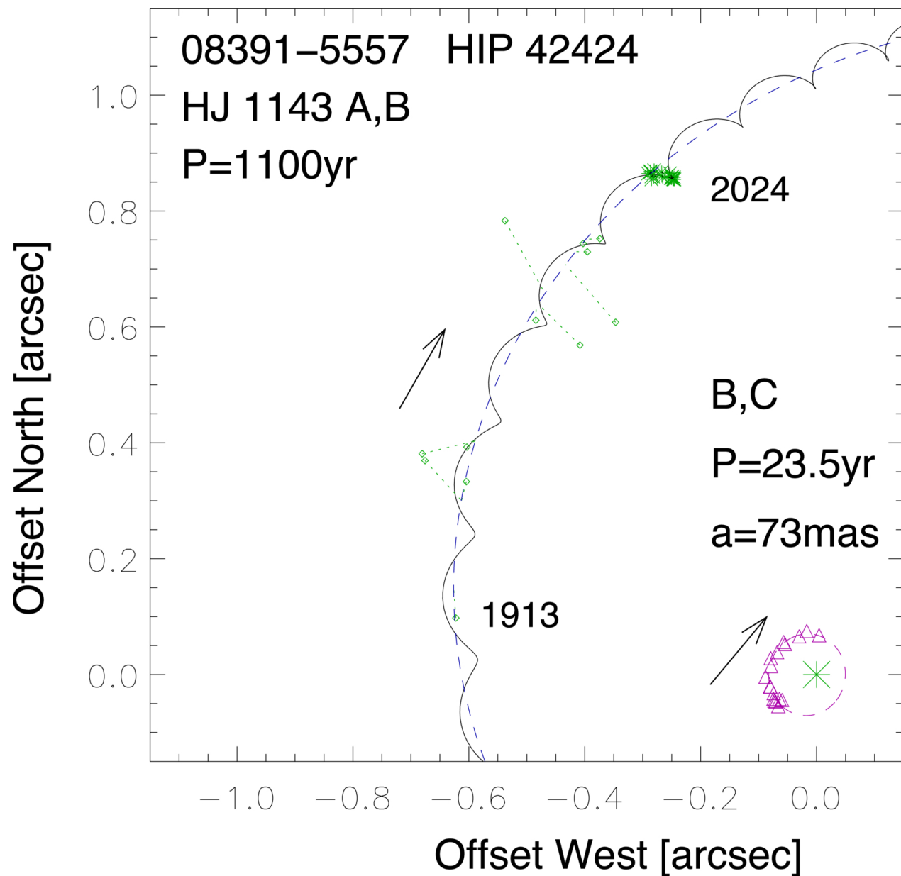
Figure 5. from Andrei Tokovinin 2026 Astron. J. 171 doi:10.3847/1538-3881/ae2fe6 https://dx.doi.org/10.3847/1538-3881/ae2fe6 © 2026. The Author(s). Published by the American Astronomical Society.
