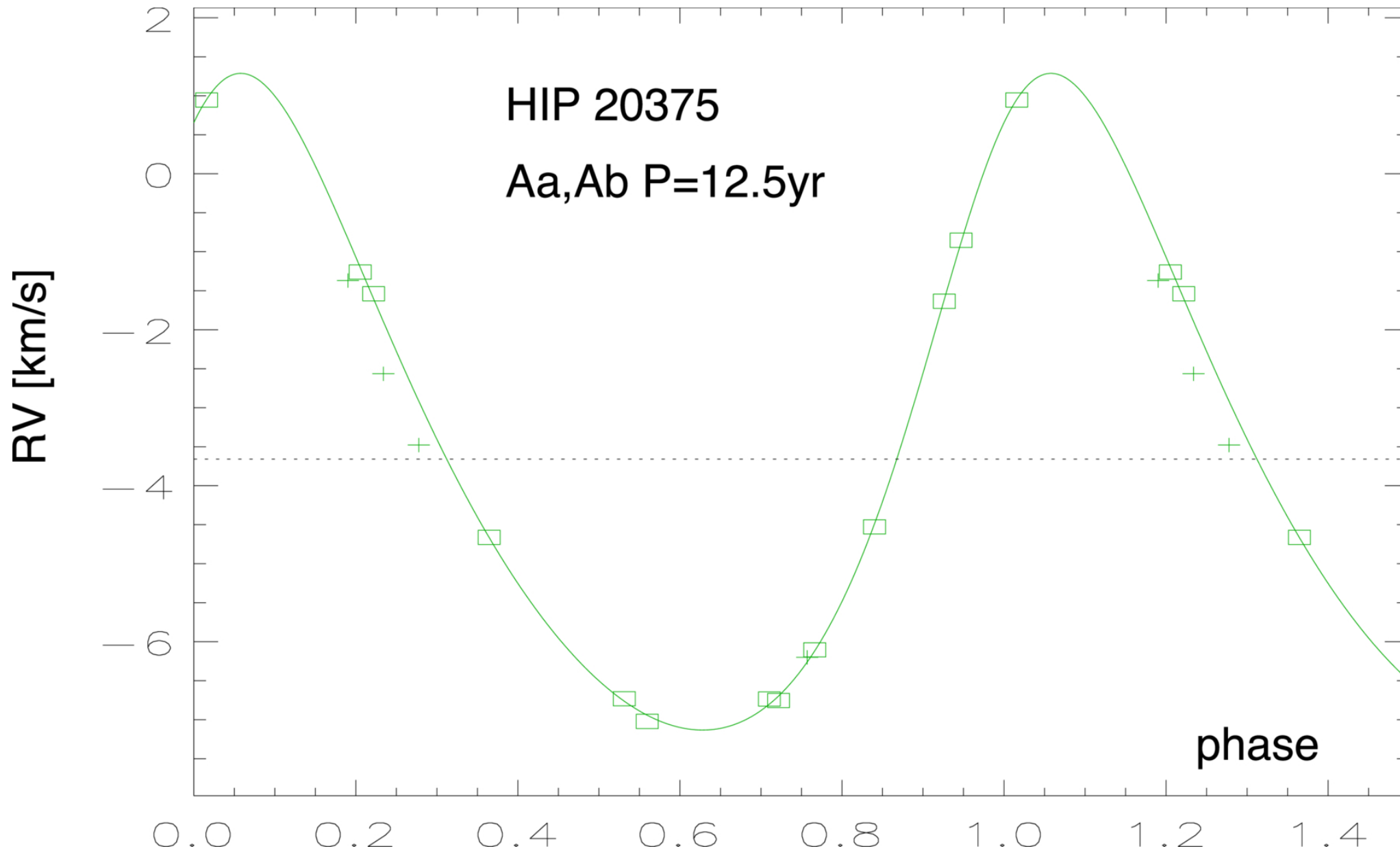
Figure 4. from Andrei Tokovinin 2026 Astron. J. 171 doi:10.3847/1538-3881/ae2fe6 https://dx.doi.org/10.3847/1538-3881/ae2fe6 © 2026. The Author(s). Published by the American Astronomical Society.
