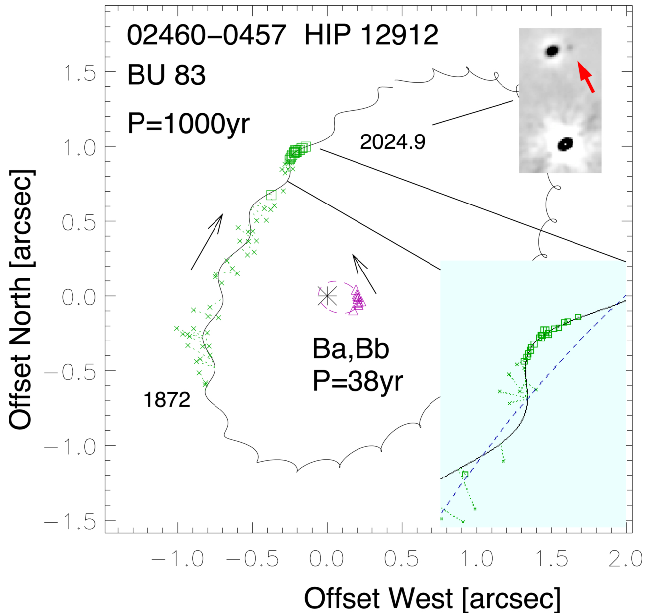
Figure 2. from Andrei Tokovinin 2026 Astron. J. 171 doi:10.3847/1538-3881/ae2fe6 https://dx.doi.org/10.3847/1538-3881/ae2fe6 © 2026. The Author(s). Published by the American Astronomical Society.
