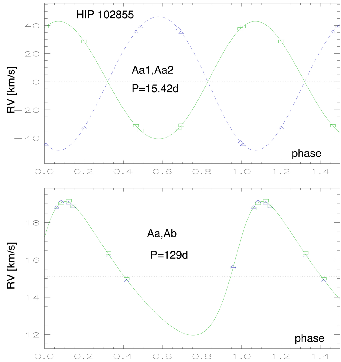
Figure 14. from Andrei Tokovinin 2026 Astron. J. 171 doi:10.3847/1538-3881/ae2fe6 https://dx.doi.org/10.3847/1538-3881/ae2fe6 © 2026. The Author(s). Published by the American Astronomical Society.
