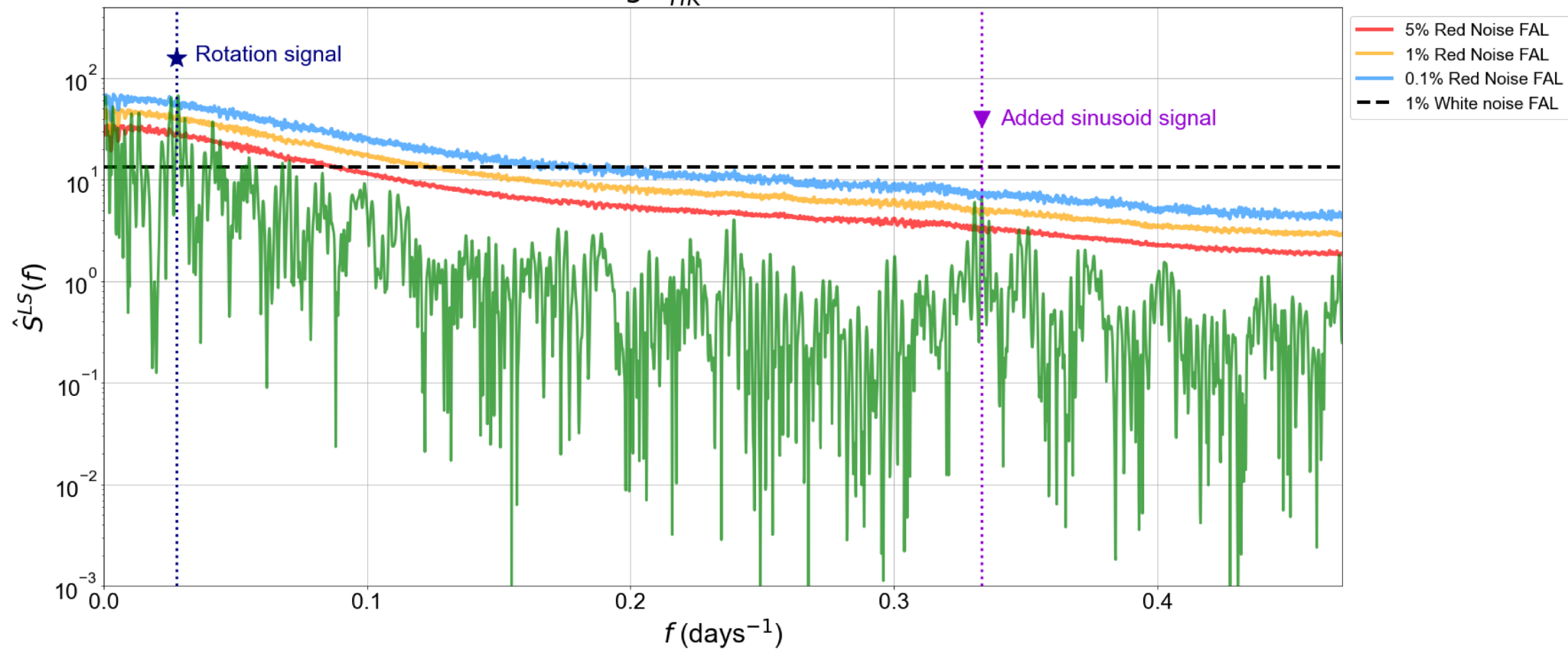
Figure 8. from Amna Ejaz et al 2026 Astron. J. 171 doi:10.3847/1538-3881/ae2fe4 https://dx.doi.org/10.3847/1538-3881/ae2fe4 © 2026. The Author(s). Published by the American Astronomical Society.
