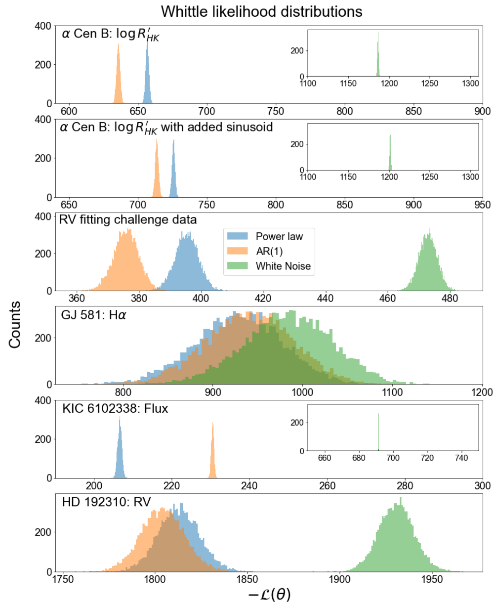
Figure 5. from Amna Ejaz et al 2026 Astron. J. 171 doi:10.3847/1538-3881/ae2fe4 https://dx.doi.org/10.3847/1538-3881/ae2fe4 © 2026. The Author(s). Published by the American Astronomical Society.
