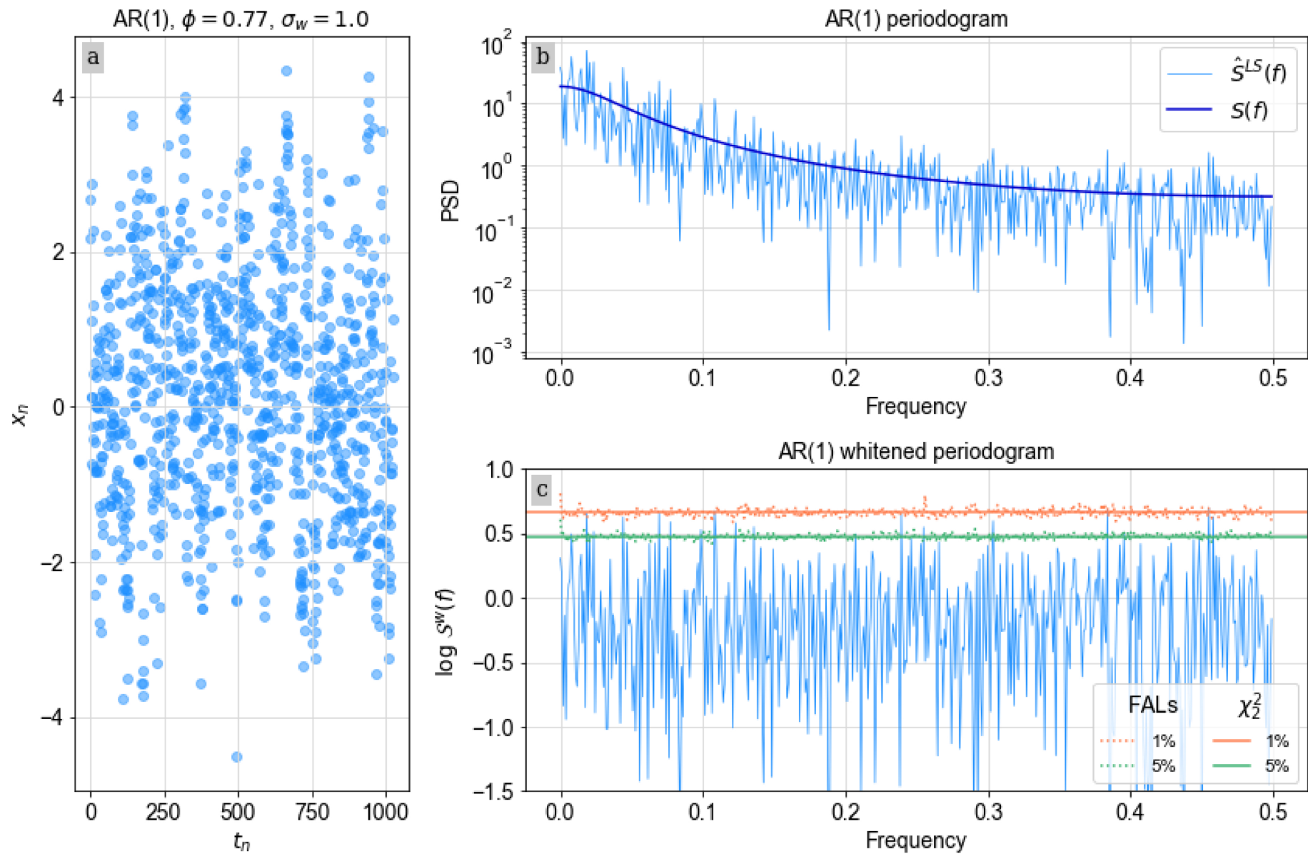
Figure 15. from Amna Ejaz et al 2026 Astron. J. 171 doi:10.3847/1538-3881/ae2fe4 https://dx.doi.org/10.3847/1538-3881/ae2fe4 © 2026. The Author(s). Published by the American Astronomical Society.
