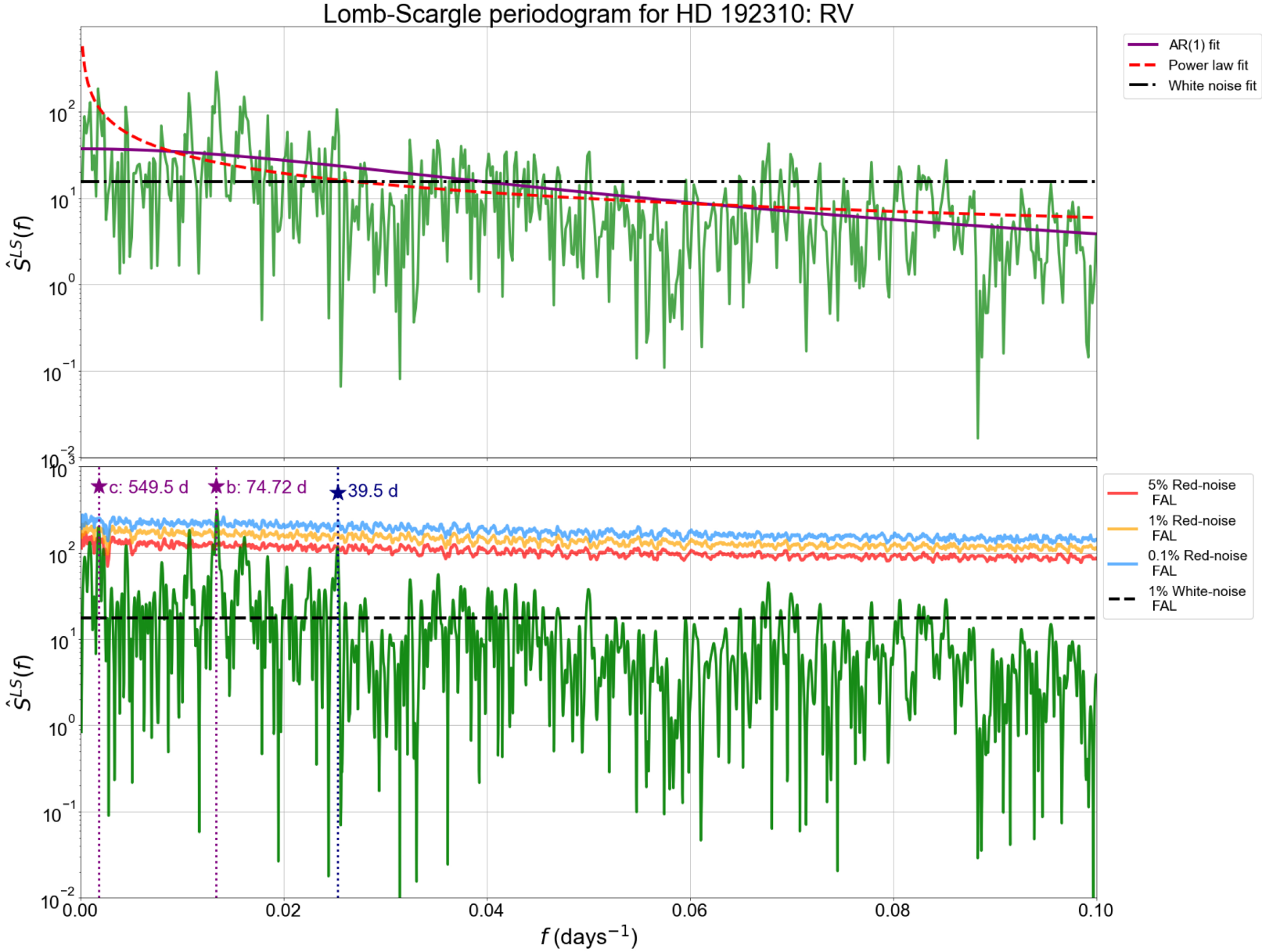
Figure 14. from Amna Ejaz et al 2026 Astron. J. 171 doi:10.3847/1538-3881/ae2fe4 https://dx.doi.org/10.3847/1538-3881/ae2fe4 © 2026. The Author(s). Published by the American Astronomical Society.
