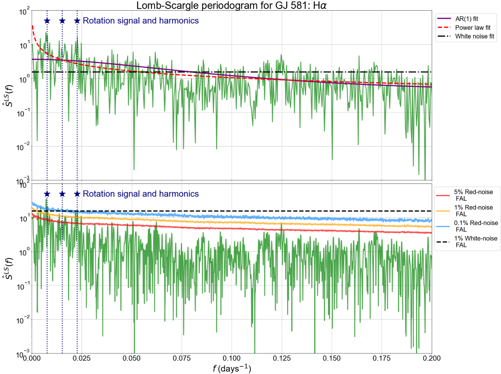
Figure 11. from Amna Ejaz et al 2026 Astron. J. 171 doi:10.3847/1538-3881/ae2fe4 https://dx.doi.org/10.3847/1538-3881/ae2fe4 © 2026. The Author(s). Published by the American Astronomical Society.
