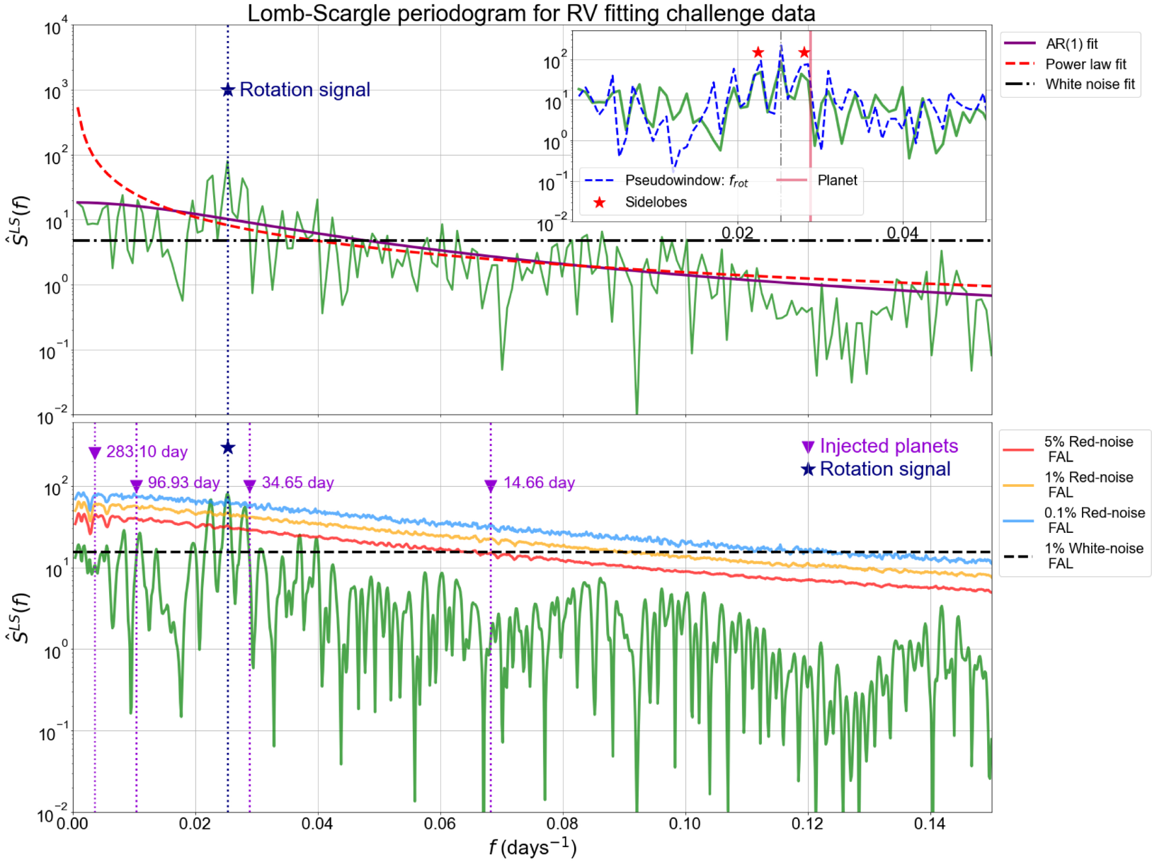
Figure 10. from Amna Ejaz et al 2026 Astron. J. 171 doi:10.3847/1538-3881/ae2fe4 https://dx.doi.org/10.3847/1538-3881/ae2fe4 © 2026. The Author(s). Published by the American Astronomical Society.
