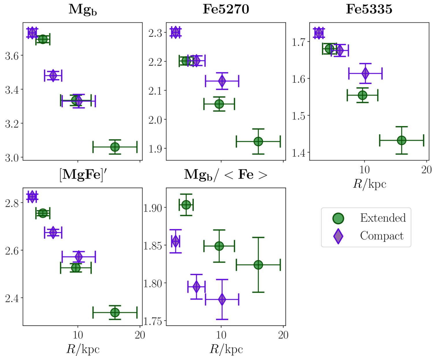
Figure 7. from Xiaoya Zhang et al 2026 Astron. J. 171 doi:10.3847/1538-3881/ae2fe1 https://dx.doi.org/10.3847/1538-3881/ae2fe1 © 2026. The Author(s). Published by the American Astronomical Society.
