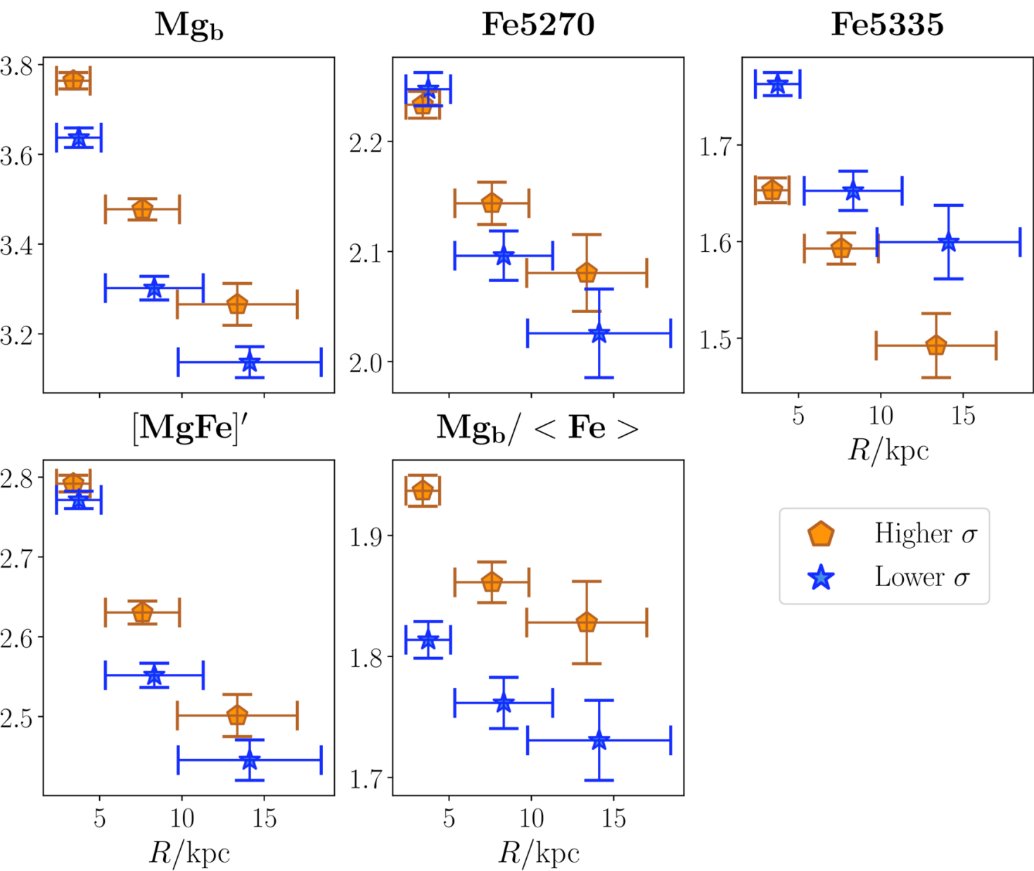
Figure 6. from Xiaoya Zhang et al 2026 Astron. J. 171 doi:10.3847/1538-3881/ae2fe1 https://dx.doi.org/10.3847/1538-3881/ae2fe1 © 2026. The Author(s). Published by the American Astronomical Society.
