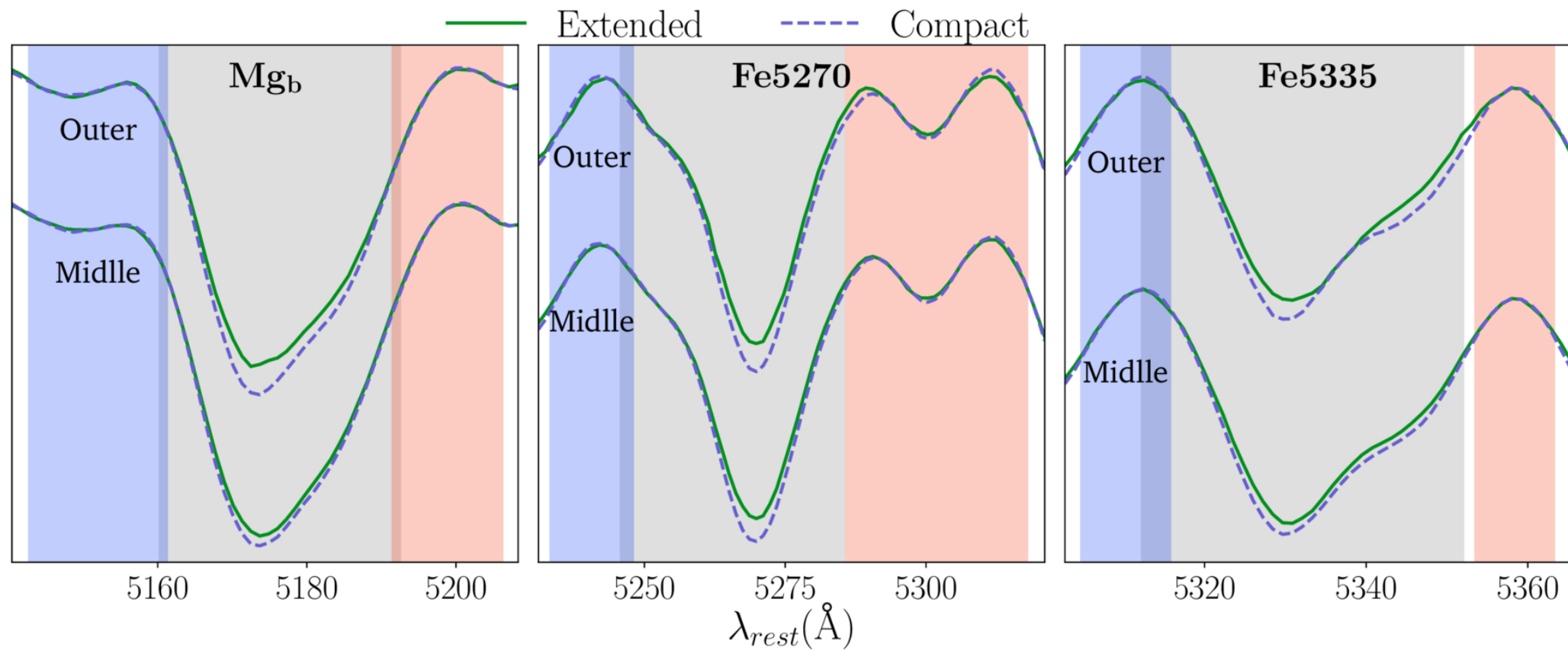
Figure 5. from Xiaoya Zhang et al 2026 Astron. J. 171 doi:10.3847/1538-3881/ae2fe1 https://dx.doi.org/10.3847/1538-3881/ae2fe1 © 2026. The Author(s). Published by the American Astronomical Society.
