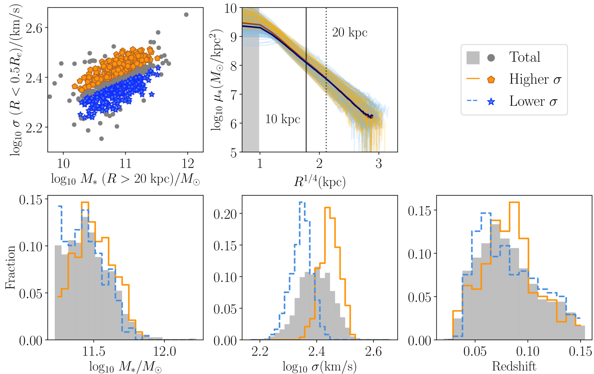
Figure 3. from Xiaoya Zhang et al 2026 Astron. J. 171 doi:10.3847/1538-3881/ae2fe1 https://dx.doi.org/10.3847/1538-3881/ae2fe1 © 2026. The Author(s). Published by the American Astronomical Society.
