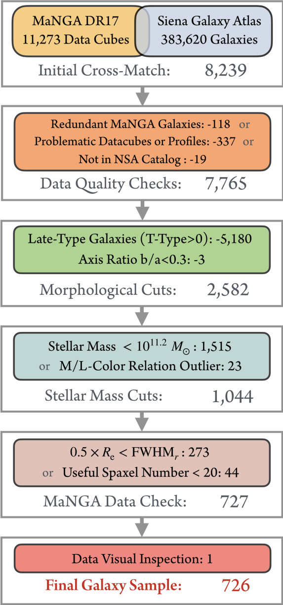
Figure 1. from Xiaoya Zhang et al 2026 Astron. J. 171 doi:10.3847/1538-3881/ae2fe1 https://dx.doi.org/10.3847/1538-3881/ae2fe1 © 2026. The Author(s). Published by the American Astronomical Society.
