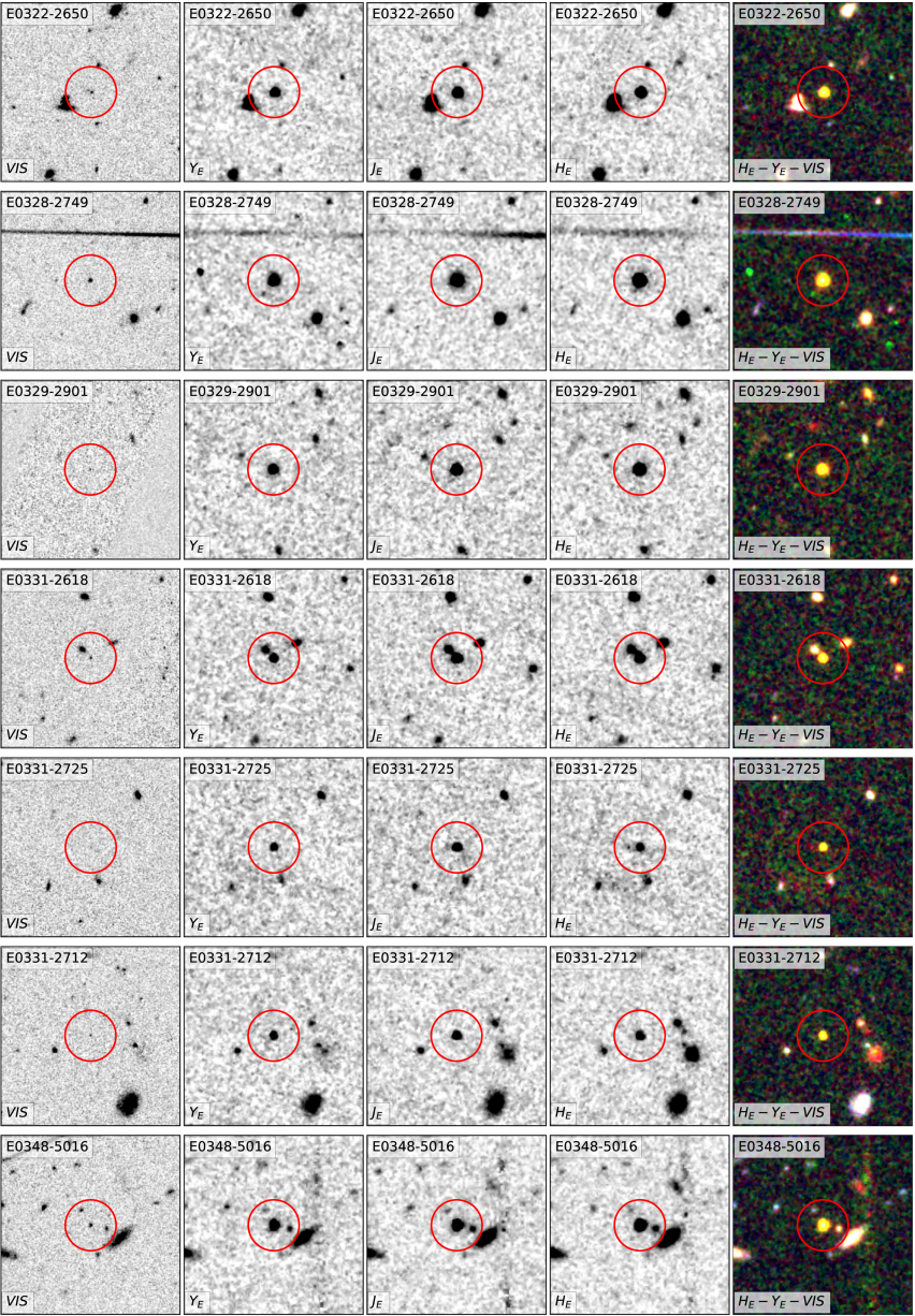
Figure 3. from Frank Kiwy et al 2026 Astron. J. 171 doi:10.3847/1538-3881/ae2fb7 https://dx.doi.org/10.3847/1538-3881/ae2fb7 © 2026. The Author(s). Published by the American Astronomical Society.
