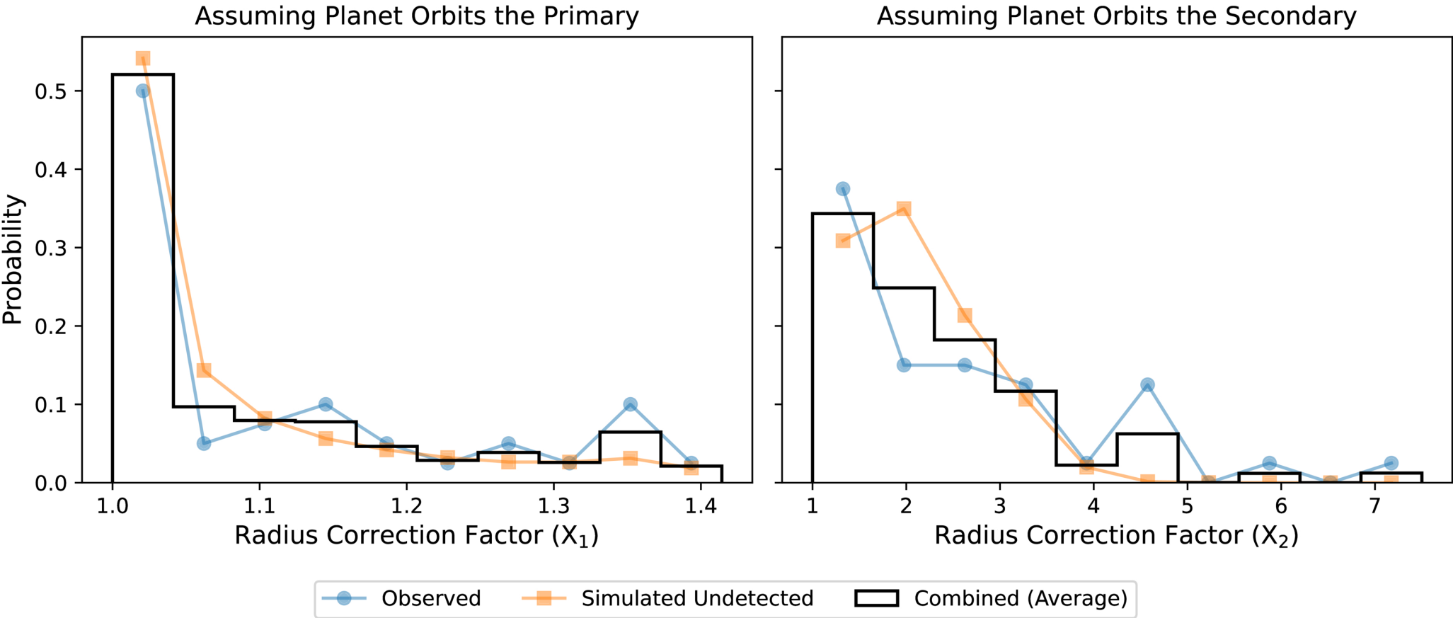
Figure 4. from Galen J. Bergsten et al 2026 Astron. J. 171 doi:10.3847/1538-3881/ae2ead https://dx.doi.org/10.3847/1538-3881/ae2ead © 2026. The Author(s). Published by the American Astronomical Society.
