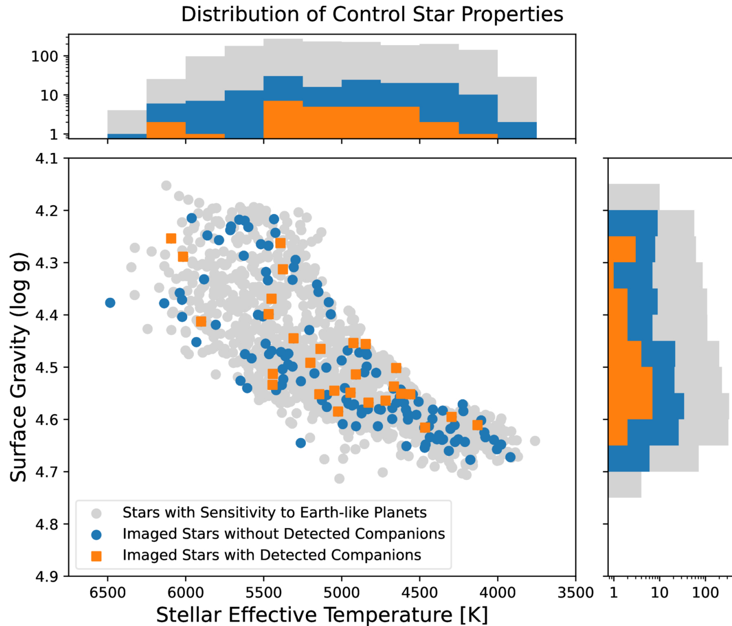
Figure 1. from Galen J. Bergsten et al 2026 Astron. J. 171 doi:10.3847/1538-3881/ae2ead https://dx.doi.org/10.3847/1538-3881/ae2ead © 2026. The Author(s). Published by the American Astronomical Society.
