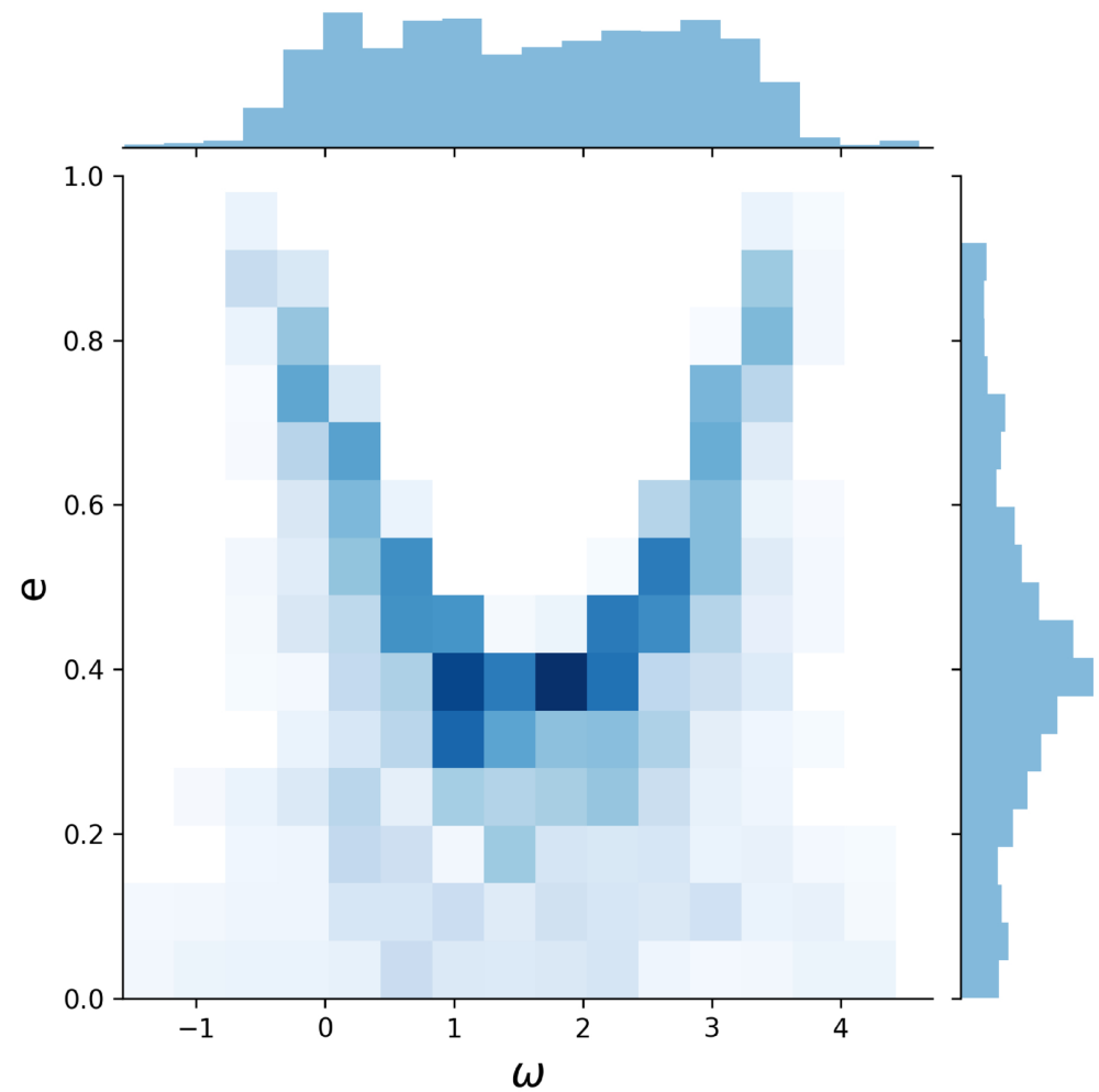
e - \omega posterior from this work
