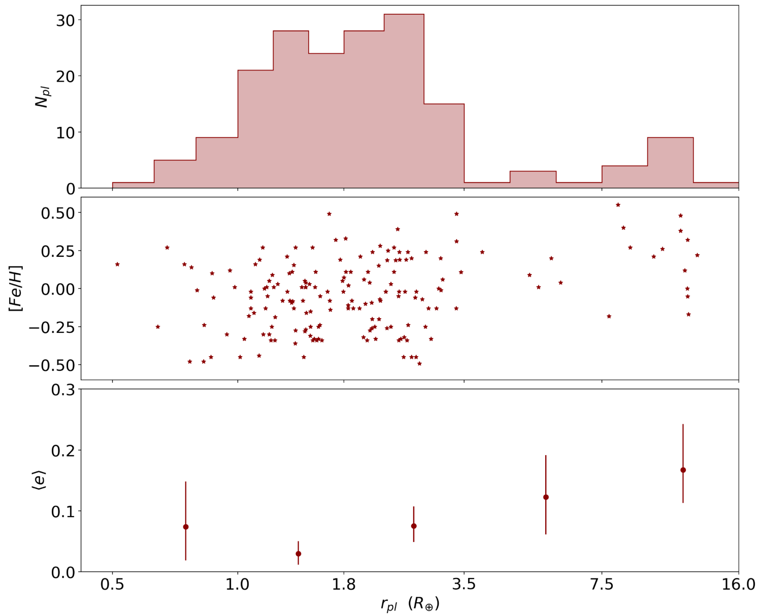
Figure 8. from Sheila Saguear et al 2026 Astron. J. 171 doi:10.3847/1538-3881/ae2d1b https://dx.doi.org/10.3847/1538-3881/ae2d1b © 2026. The Author(s). Published by the American Astronomical Society.
