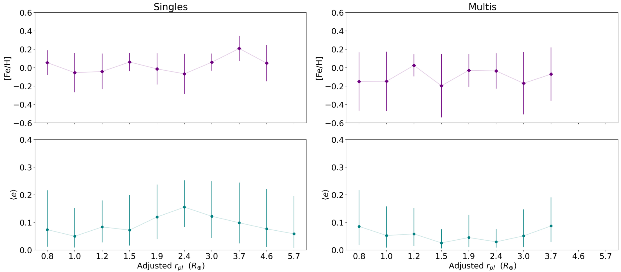
Figure 7. from Sheila Sagar et al 2026 Astron. J. 171 doi:10.3847/1538-3881/ae2d1b https://dx.doi.org/10.3847/1538-3881/ae2d1b © 2026. The Author(s). Published by the American Astronomical Society.
