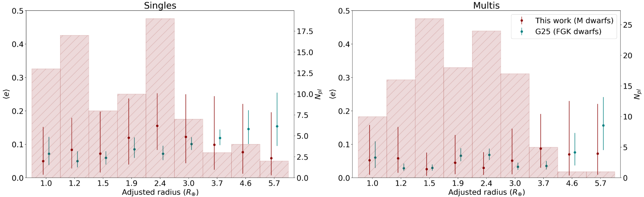
Figure 5. from Sheila Sagar et al 2026 Astron. J. 171 doi:10.3847/1538-3881/ae2d1b https://dx.doi.org/10.3847/1538-3881/ae2d1b © 2026. The Author(s). Published by the American Astronomical Society.
