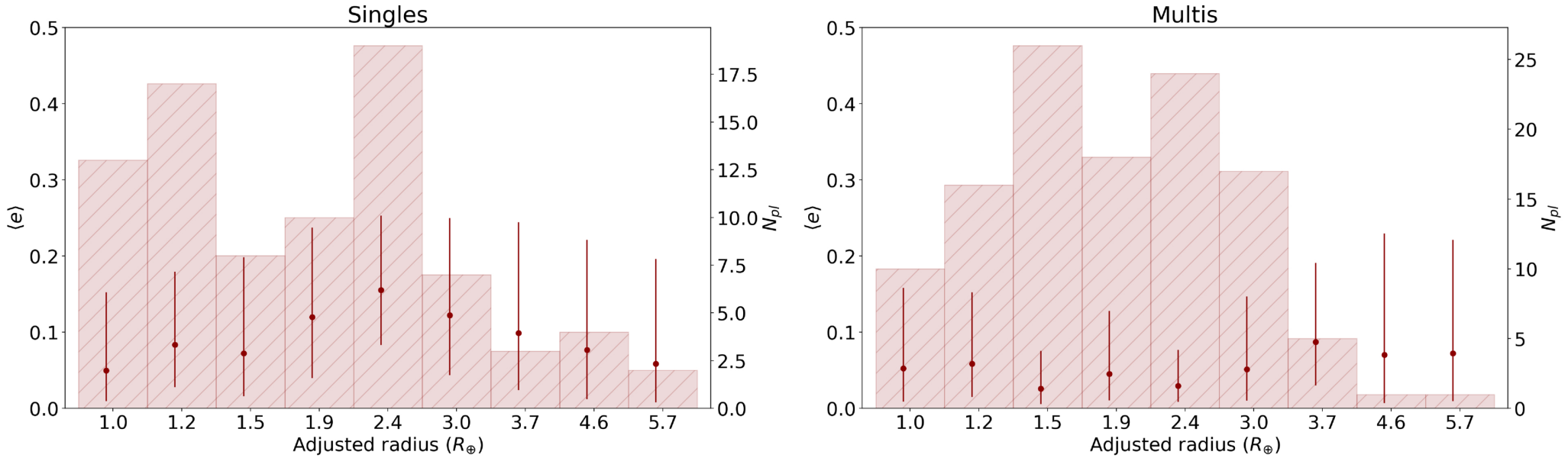
Figure 3. from Sheila Sague et al 2026 Astron. J. 171 doi:10.3847/1538-3881/ae2d1b https://dx.doi.org/10.3847/1538-3881/ae2d1b © 2026. The Author(s). Published by the American Astronomical Society.
