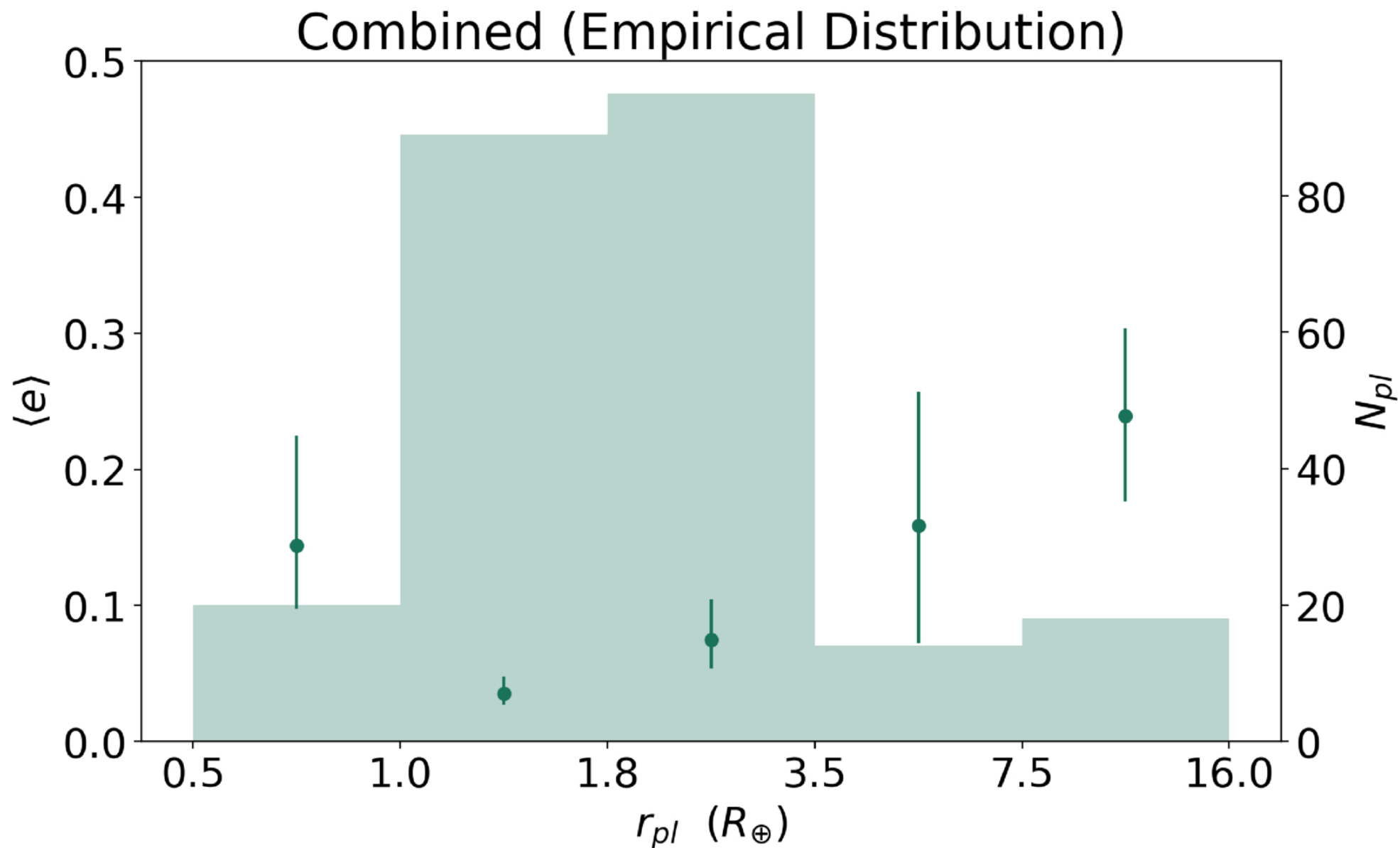
Figure 13. from Sheila Sagar et al 2026 Astron. J. 171 doi:10.3847/1538-3881/ae2d1b https://dx.doi.org/10.3847/1538-3881/ae2d1b © 2026. The Author(s). Published by the American Astronomical Society.
