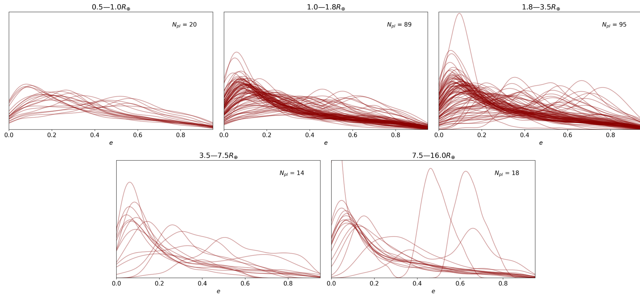
Figure 11. from Sheila Saguear et al 2026 Astron. J. 171 doi:10.3847/1538-3881/ae2d1b https://dx.doi.org/10.3847/1538-3881/ae2d1b © 2026. The Author(s). Published by the American Astronomical Society.
