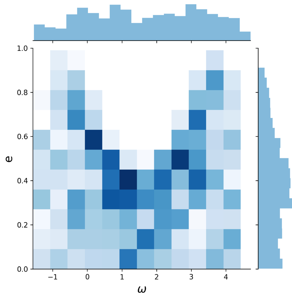
KOI 247.01 (First 9 Long-Cadence Transits)
