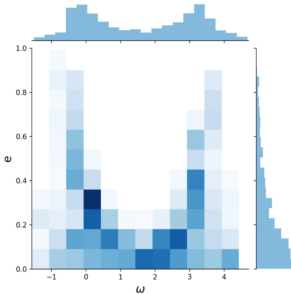
TOI 555.01 (First 9 Transits)
