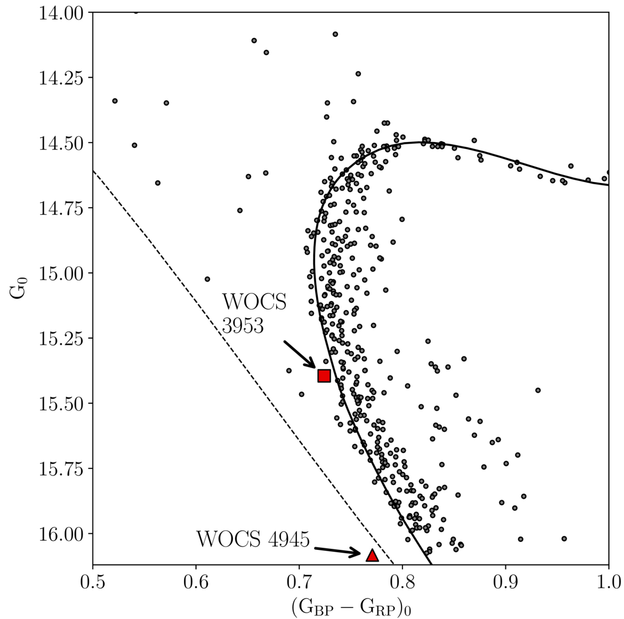
Figure 9. from Ritvik Sai Narayan et al 2026 Astron. J. 171 doi:10.3847/1538-3881/ae2d14 https://dx.doi.org/10.3847/1538-3881/ae2d14 © 2026. The Author(s). Published by the American Astronomical Society.
