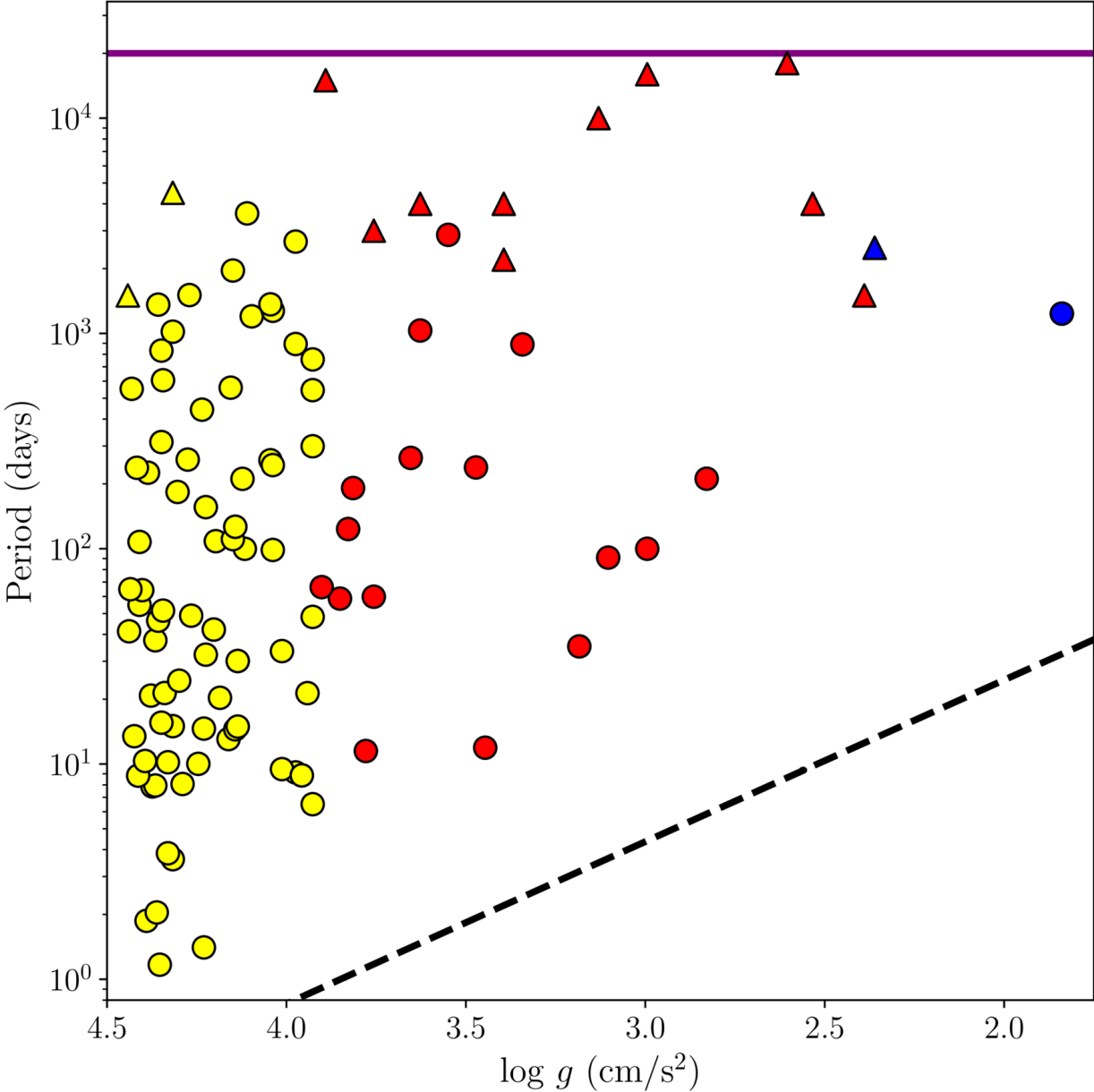
Figure 8. from Ritvik Sai Narayan et al 2026 Astron. J. 171 doi:10.3847/1538-3881/ae2d14 https://dx.doi.org/10.3847/1538-3881/ae2d14 © 2026. The Author(s). Published by the American Astronomical Society.
