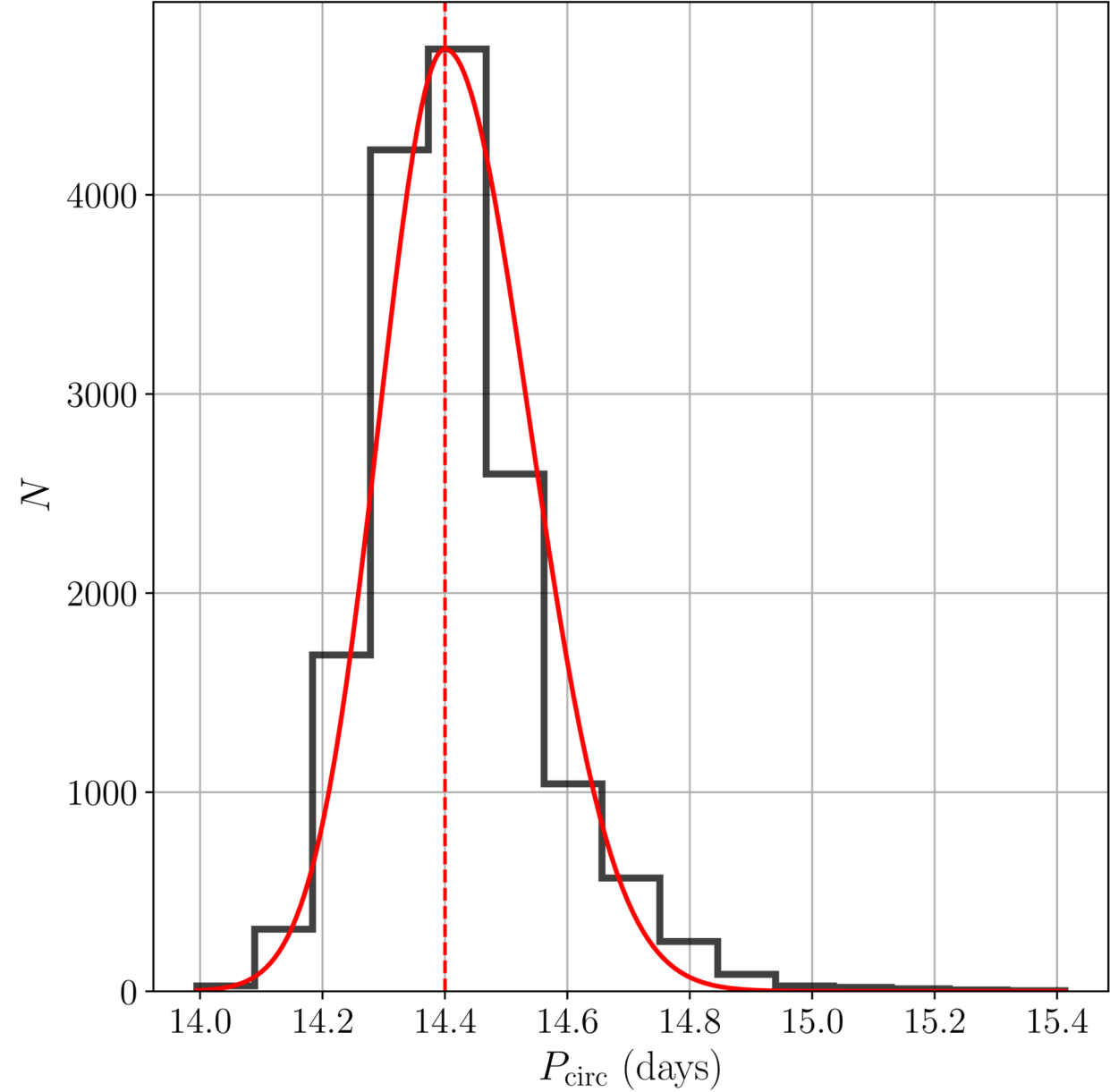
Figure 7. from Ritvik Sai Narayan et al 2026 Astron. J. 171 doi:10.3847/1538-3881/ae2d14 https://dx.doi.org/10.3847/1538-3881/ae2d14 © 2026. The Author(s). Published by the American Astronomical Society.
