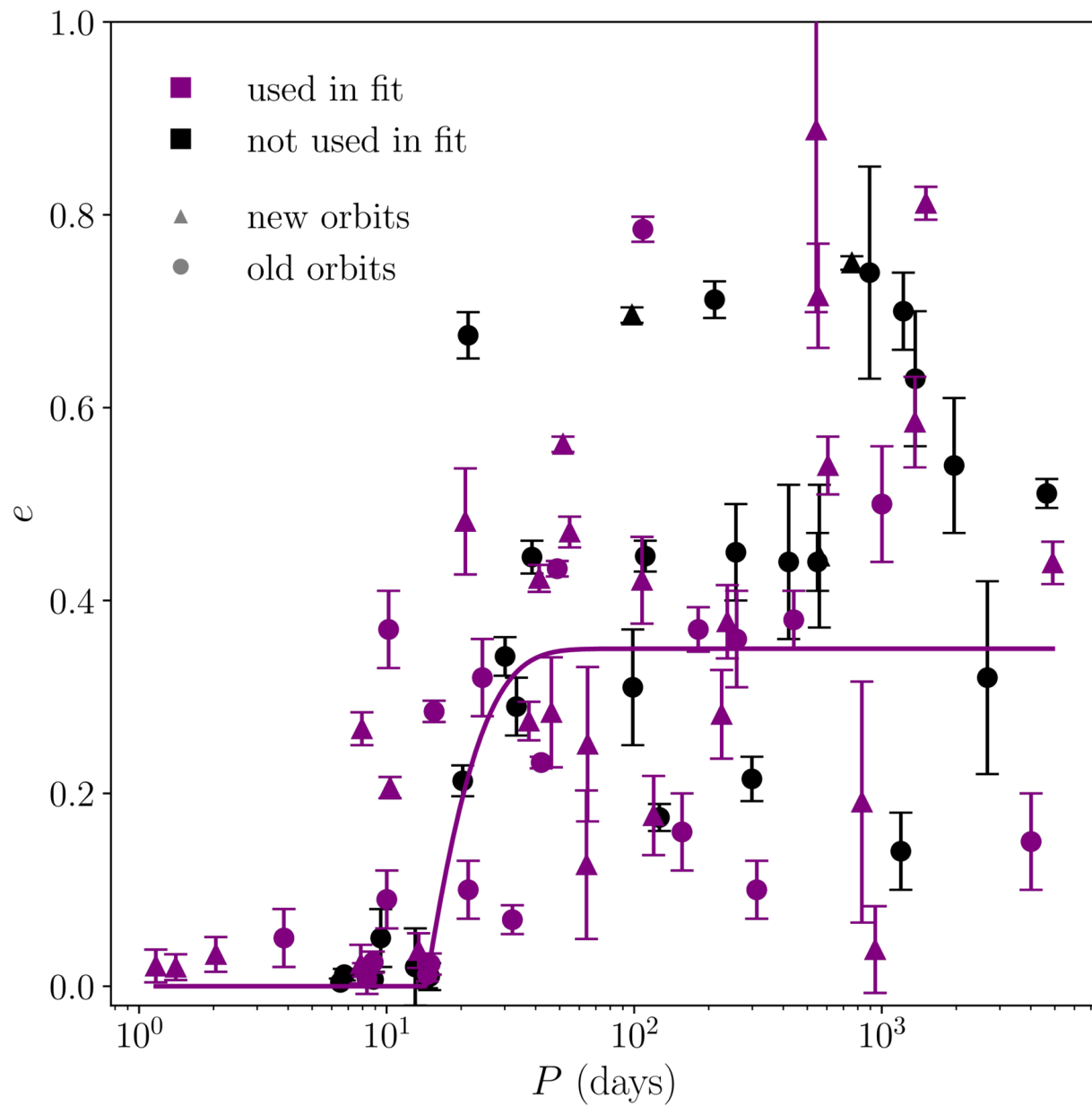
Figure 6. from Ritvik Sai Narayan et al 2026 Astron. J. 171 doi:10.3847/1538-3881/ae2d14 https://dx.doi.org/10.3847/1538-3881/ae2d14 © 2026. The Author(s). Published by the American Astronomical Society.
