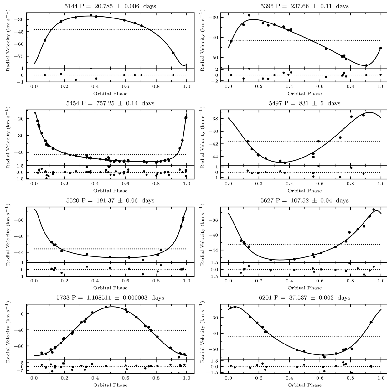
Figure 5. from Ritvik Sai Narayan et al 2026 Astron. J. 171 doi:10.3847/1538-3881/ae2d14 https://dx.doi.org/10.3847/1538-3881/ae2d14 © 2026. The Author(s). Published by the American Astronomical Society.
