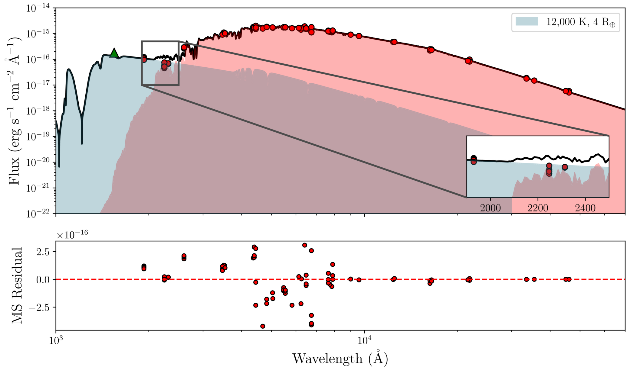
Figure 10. from Ritvik Sai Narayan et al 2026 Astron. J. 171 doi:10.3847/1538-3881/ae2d14 https://dx.doi.org/10.3847/1538-3881/ae2d14 © 2026. The Author(s). Published by the American Astronomical Society.
