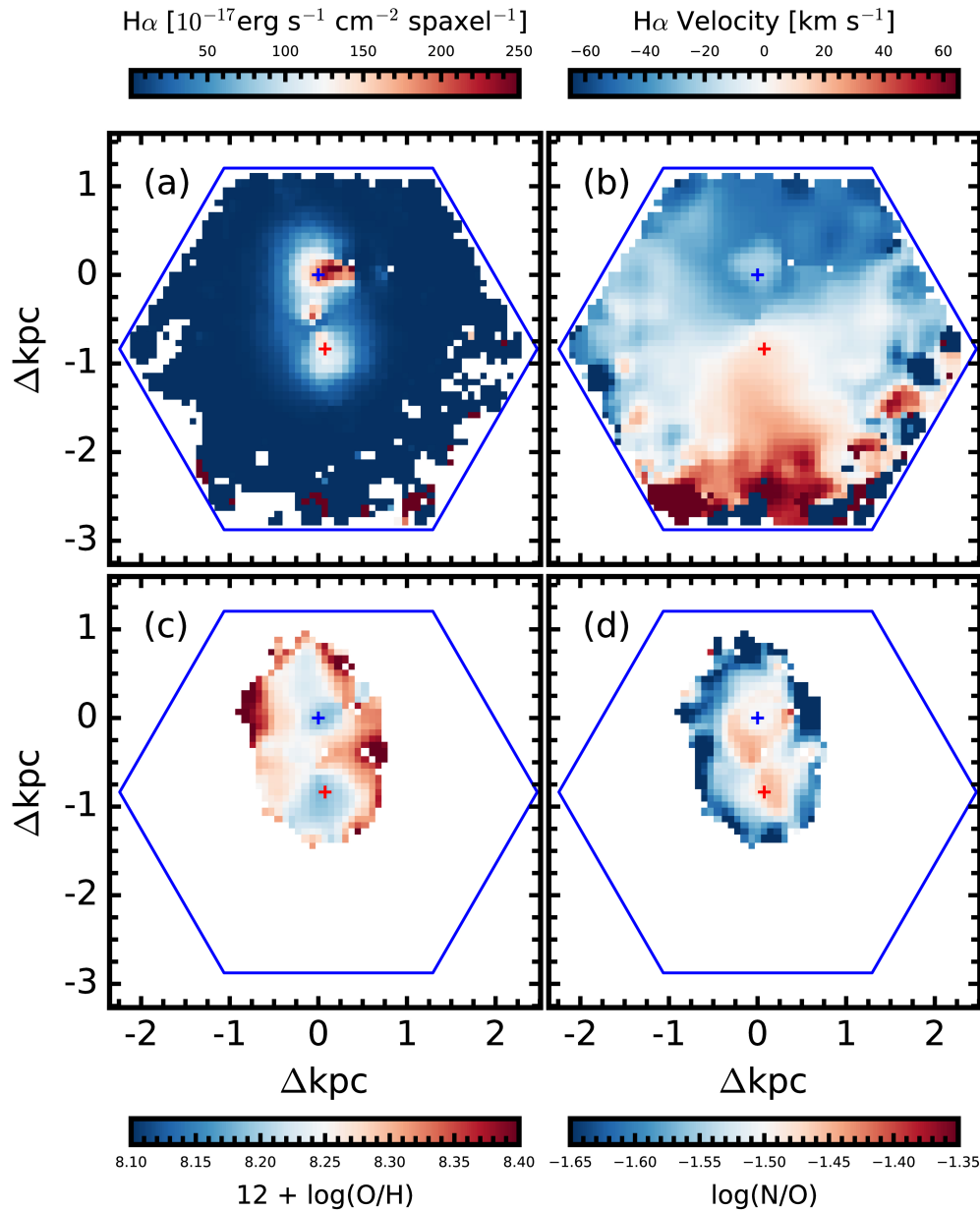
Figure 6. from Youngdae Lee 2026 Astron. J. 171 doi:10.3847/1538-3881/ae2c5b https://dx.doi.org/10.3847/1538-3881/ae2c5b © 2026. The Author(s). Published by the American Astronomical Society.
