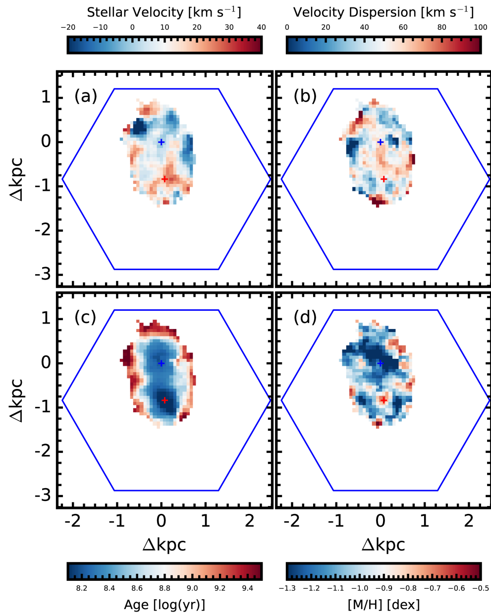
Figure 5. from Youngdae Lee 2026 Astron. J. 171 doi:10.3847/1538-3881/ae2c5b https://dx.doi.org/10.3847/1538-3881/ae2c5b © 2026. The Author(s). Published by the American Astronomical Society.
