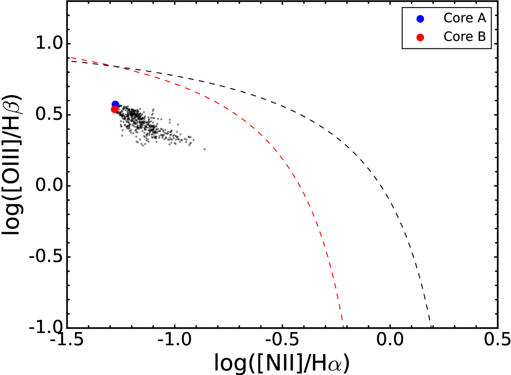
Figure 3. from Youngdae Lee 2026 Astron. J. 171 doi:10.3847/1538-3881/ae2c5b https://dx.doi.org/10.3847/1538-3881/ae2c5b © 2026. The Author(s). Published by the American Astronomical Society.
