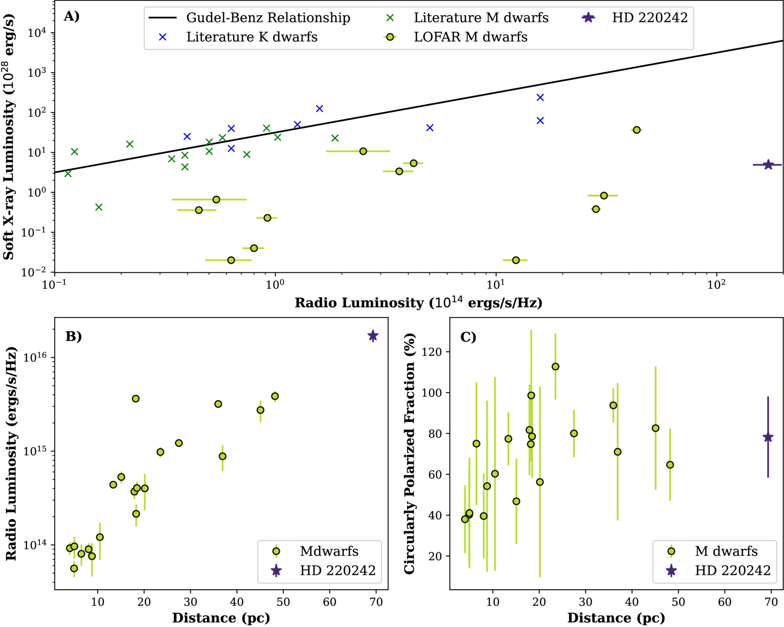
Figure 4. from Megan Delamer et al 2026 Astron. J. 171 doi:10.3847/1538-3881/ae2c55 https://dx.doi.org/10.3847/1538-3881/ae2c55 © 2026. The Author(s). Published by the American Astronomical Society.
