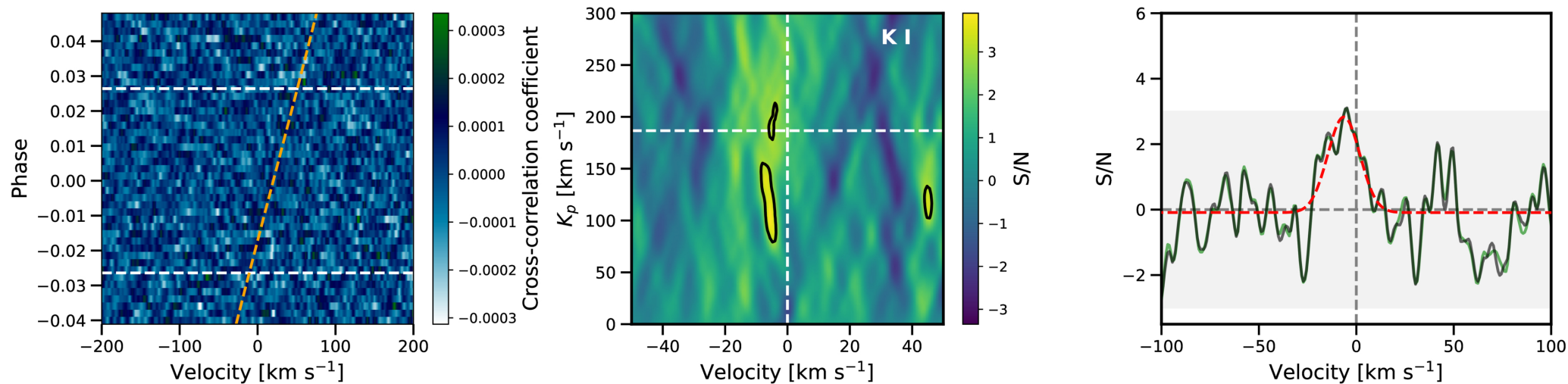
Figure 8. from Tianjun Gan et al 2026 Astron. J. 171 doi:10.3847/1538-3881/ae2add https://dx.doi.org/10.3847/1538-3881/ae2add © 2026. The Author(s). Published by the American Astronomical Society.
