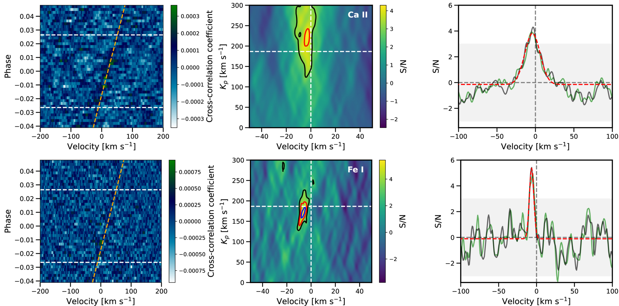
Figure 7. from Tianjun Gan et al 2026 Astron. J. 171 doi:10.3847/1538-3881/ae2add https://dx.doi.org/10.3847/1538-3881/ae2add © 2026. The Author(s). Published by the American Astronomical Society.
