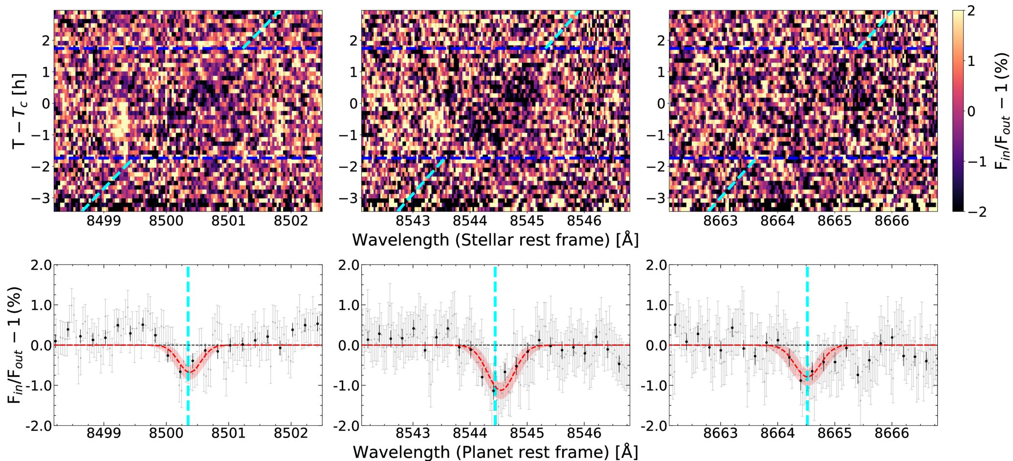
Figure 6. from Tianjun Gan et al 2026 Astron. J. 171 doi:10.3847/1538-3881/ae2add https://dx.doi.org/10.3847/1538-3881/ae2add © 2026. The Author(s). Published by the American Astronomical Society.
