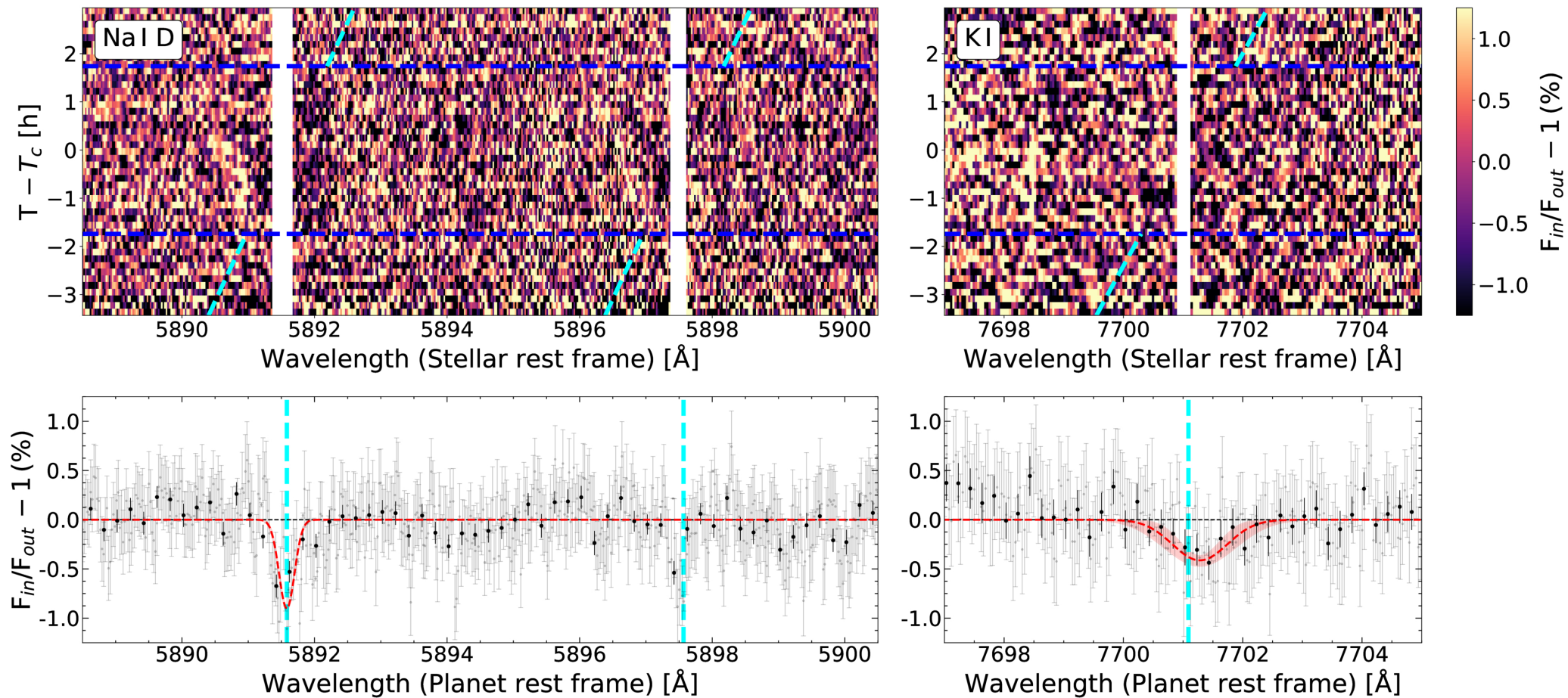
Figure 5. from Tianjun Gan et al 2026 Astron. J. 171 doi:10.3847/1538-3881/ae2add https://dx.doi.org/10.3847/1538-3881/ae2add © 2026. The Author(s). Published by the American Astronomical Society.
