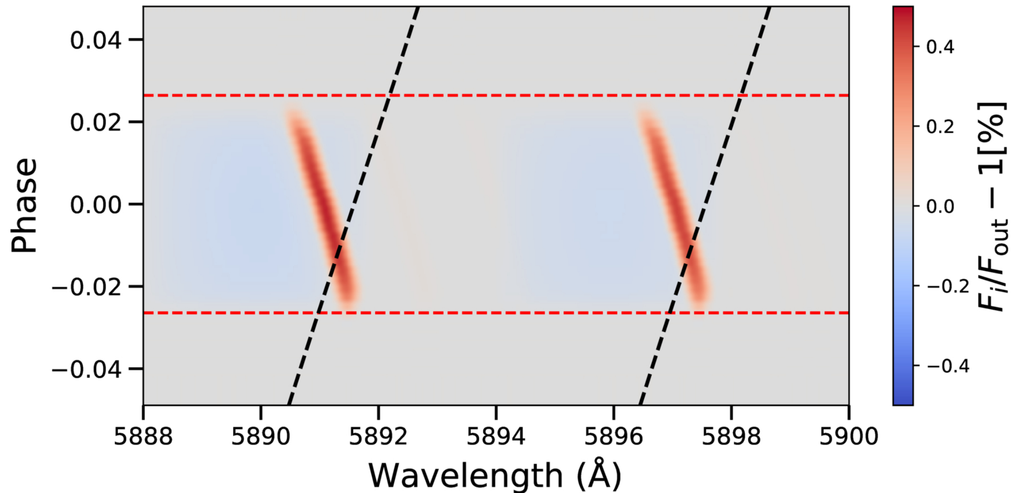
Figure 2. from Tianjun Gan et al 2026 Astron. J. 171 doi:10.3847/1538-3881/ae2add https://dx.doi.org/10.3847/1538-3881/ae2add © 2026. The Author(s). Published by the American Astronomical Society.
