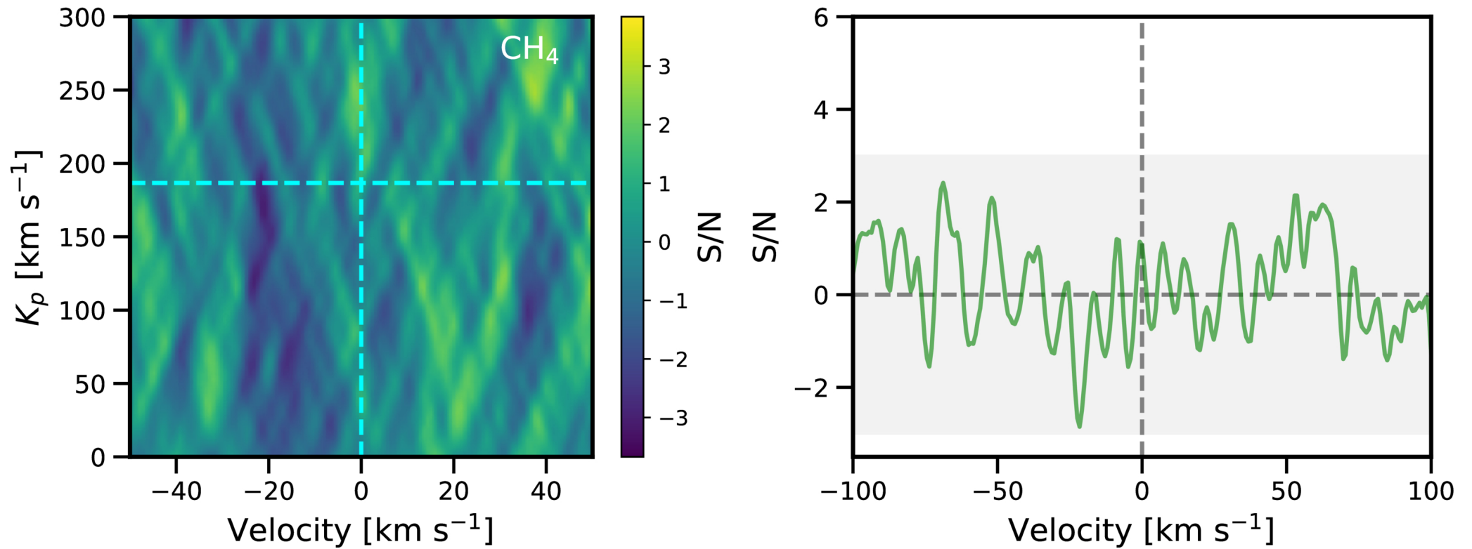
Figure A4. Nondetections of molecular species from Tianjun Gan et al 2026 Astron. J. 171 doi:10.3847/1538-3881/ae2add https://dx.doi.org/10.3847/1538-3881/ae2add © 2026. The Author(s). Published by the American Astronomical Society.
