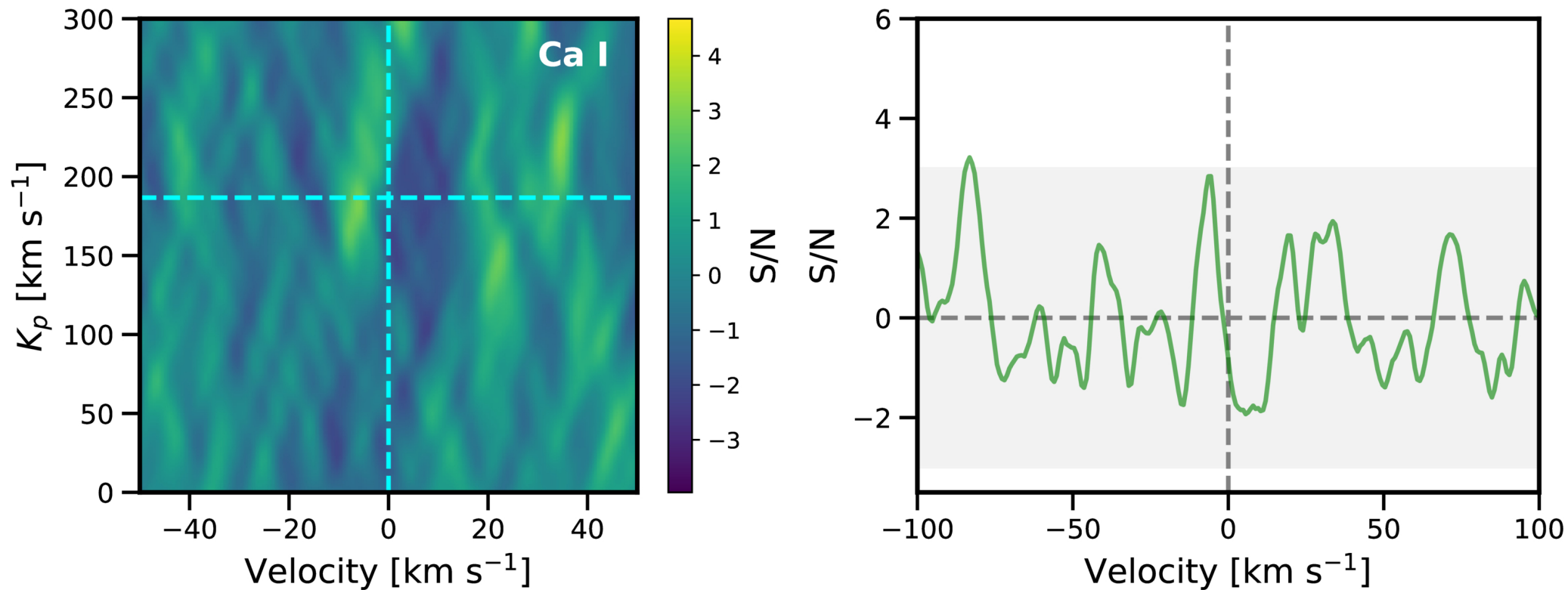
Figure A3. Nondetections of atomic species from Tianjun Gan et al 2026 Astron. J. 171 doi:10.3847/1538-3881/ae2add https://dx.doi.org/10.3847/1538-3881/ae2add © 2026. The Author(s). Published by the American Astronomical Society.
