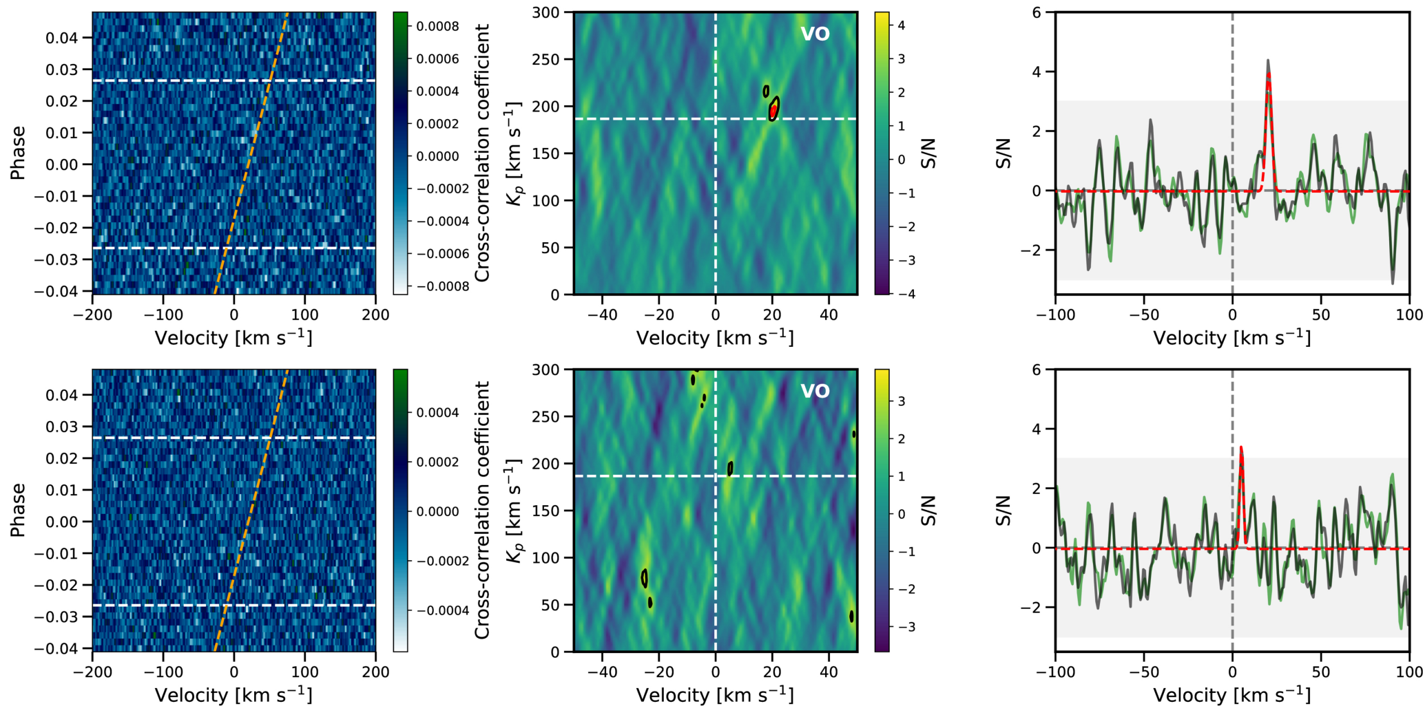
Figure A2. from Tianjun Gan et al 2026 Astron. J. 171 doi:10.3847/1538-3881/ae2add https://dx.doi.org/10.3847/1538-3881/ae2add © 2026. The Author(s). Published by the American Astronomical Society.
