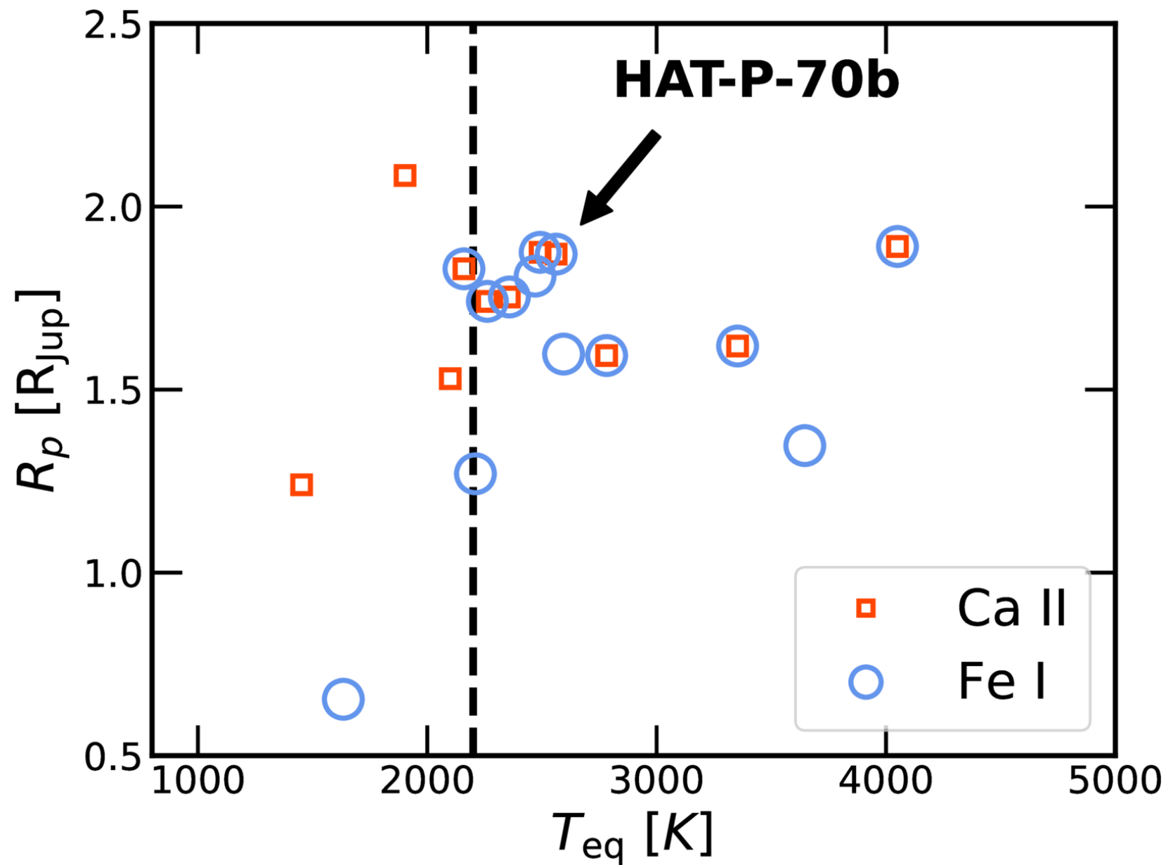
Figure 11. from Tianjun Gan et al 2026 Astron. J. 171 doi:10.3847/1538-3881/ae2add https://dx.doi.org/10.3847/1538-3881/ae2add © 2026. The Author(s). Published by the American Astronomical Society.
