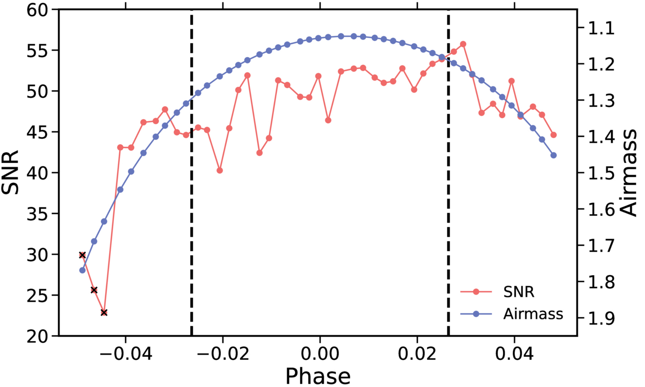
Figure 1. from Tianjun Gan et al 2026 Astron. J. 171 doi:10.3847/1538-3881/ae2add https://dx.doi.org/10.3847/1538-3881/ae2add © 2026. The Author(s). Published by the American Astronomical Society.
