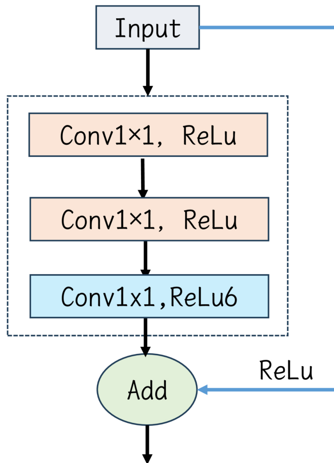
(a) Residuals
