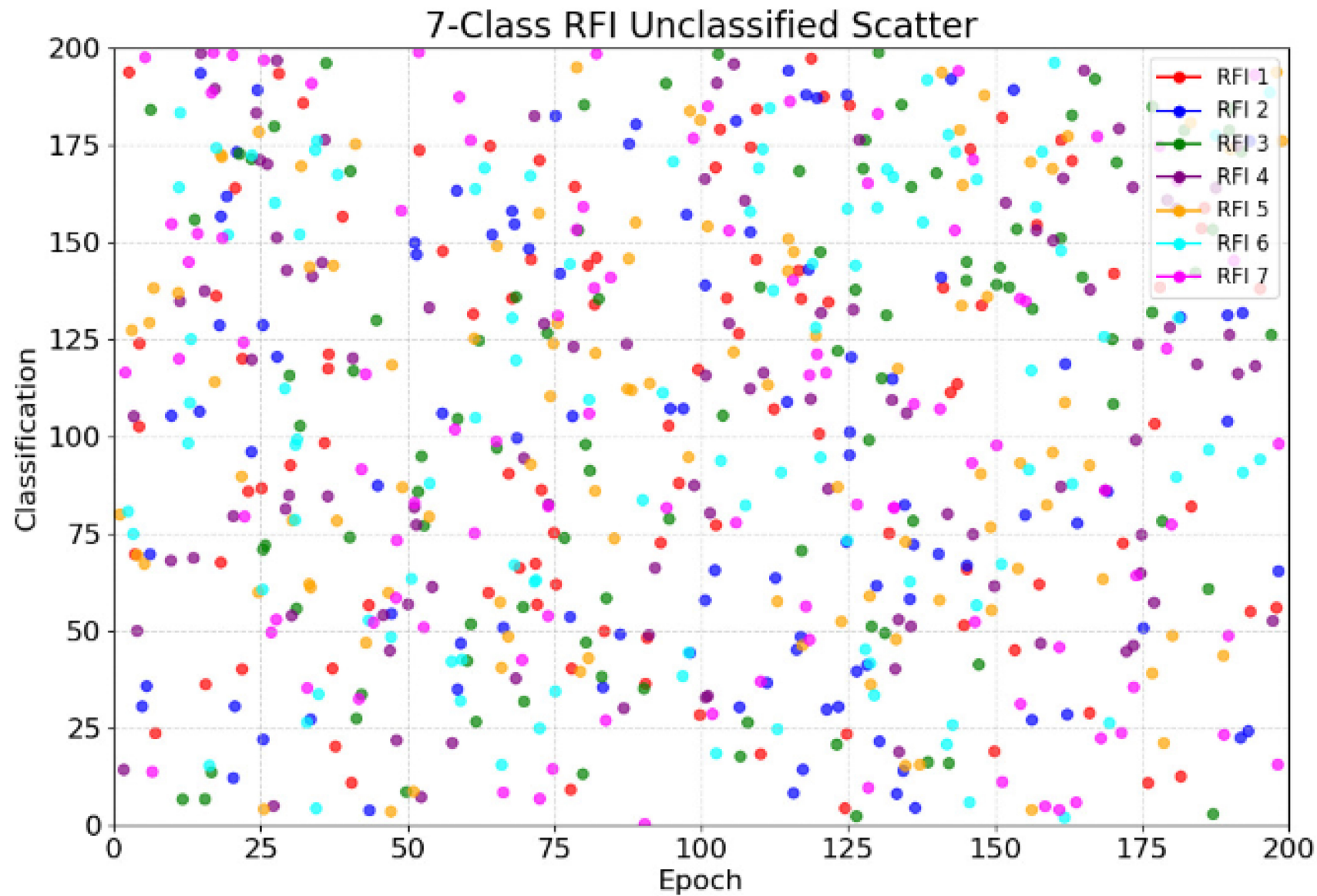
Figure 12. from Wenna Cai et al 2026 Astron. J. 171 doi:10.3847/1538-3881/ae2ad5 https://dx.doi.org/10.3847/1538-3881/ae2ad5 © 2026. The Author(s). Published by the American Astronomical Society.
